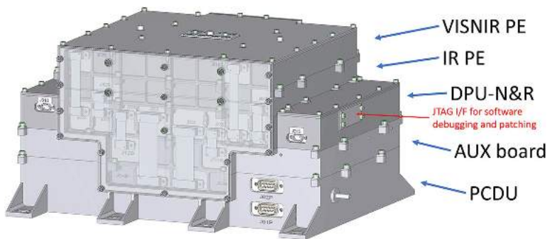
Fig. 20 Scheme showing the different electronics boards within their housing. See text for acronyms
