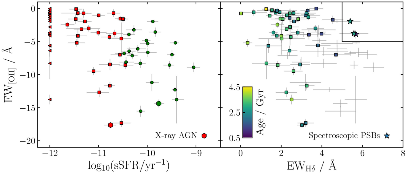
Figure 6. The distribution of [O II] emission in our sample. The left-hand panel shows EW_{[O II]} versus sSFR: symbols and colours are as defined in Fig. 4, except for galaxies with \log_{10}(sSFR/yr^{-1}) < -12 , which are shown as triangles, indicating an upper limit. Additionally, objects detected in the Chandra seven megasecond catalogue of Luo et al. (2017) are shown as hexagons (see Section 5.7). The right-hand panel shows the EW_{H\delta} versus EW_{[O II]} parameter space typically used to select post-starburst galaxies. Quiescent galaxies are coloured by mass-weighted age, green-valley galaxies are shown with grey errorbars. Commonly used spectroscopic PSB selection criteria are shown with solid lines (e.g. Tran et al. 2003; Maltby et al. 2016). Galaxies which meet these criteria are shown as stars (see Section 5.6).
