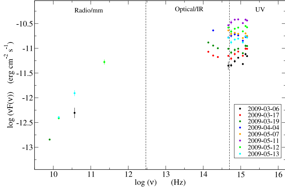
Fig. 11.— Radio to UV SEDs built using only data simultaneous within a daily time span.
