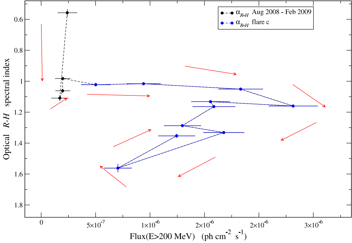
Fig. 23.— Optical R-H spectral index vs. the LAT Flux above 200 MeV. The black points refer to the 2008 August to 2009 February period, and are poorly sampled to be used to investigate the optical/ \gamma -ray connection. The blue points overlap mainly the flare c , in particular the subflare peaking at about MJD 54909 (see fig. 2, panel d). The red arrows shows the chronological sequence.
