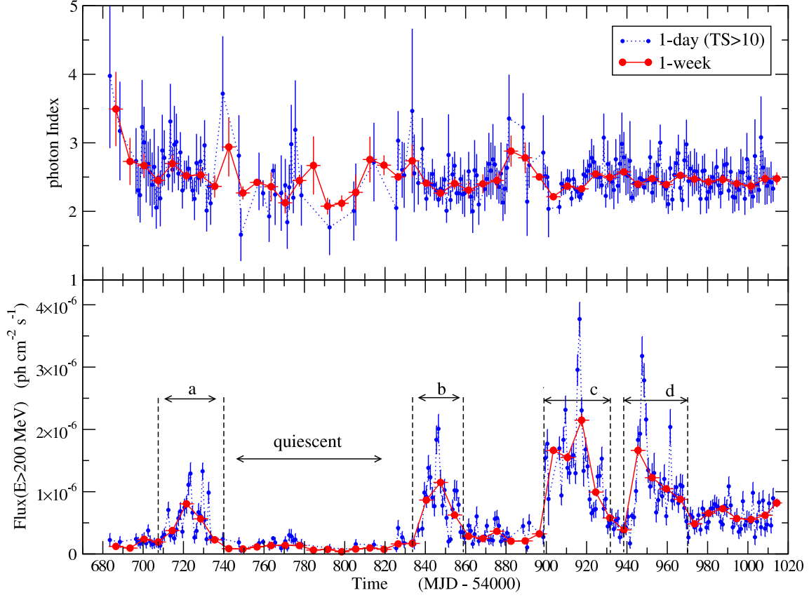
Fig. 1.— Upper Panel: the \gamma -ray photon index ( \alpha_\gamma ), as a function of the time, for weekly and daily binning. In case of daily binning only observations with a Test Statistic > 10 are taken into account. The Test Statistic is defined as TS = -2 \text{Log}(L0/L1) , where L1 and L0 are the likelihood when the source is included or not. Lower Panel: weekly, and daily (TS >10 ) fluxes light curve.
