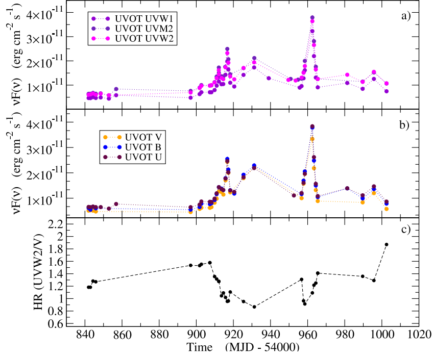
Fig. 13.— Panels a,b: UVOT light curves. Panel c: Hardness ratio of the UVOT spectra (UVW2/UVV) evaluated as a function of the time.
