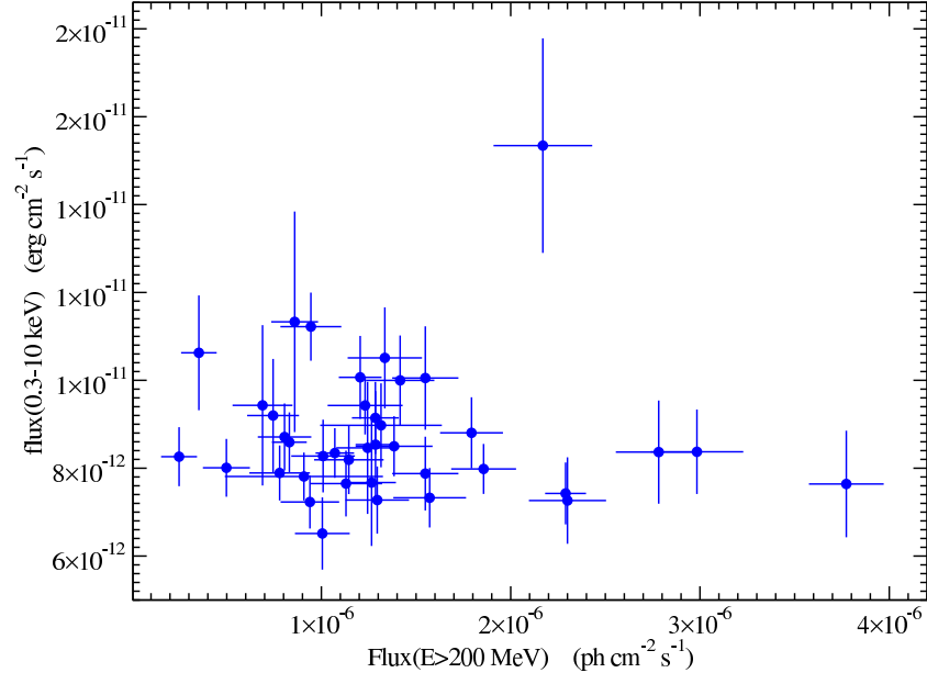
Fig. 10.— Scatter plot of the XRT flux in the 0.3-10 keV band vs. the Fermi -LAT flux (E > 200 MeV).
