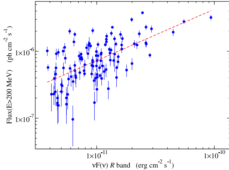
Fig. 19.— Scatter plot of the Fermi -LAT flux( E > 200 MeV) vs the \nu F(\nu) in the optical R band, using the time-shifted fluxes reported in Fig 18 . The dashed line represent the best fit by means of power-law model. The correlation coefficient in this case increases to r = 0.62 with a 95% confidence interval 0.57 \leq r \leq 0.66 .
