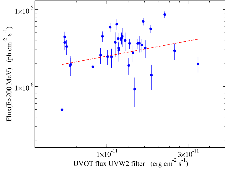
Fig. 14.— Scatter plot of the Fermi -LAT flux ( E > 200 \text{ MeV} ) vs. the UVOT \nu F(\nu) in the UVW2 filter. The red dashed line represents the best-fit power law model. The correlation coefficient of the logarithm of the UV and \gamma -ray fluxes is r = 0.2 with a 95% confidence interval of 0.05 \leq r \leq 0.34 .
