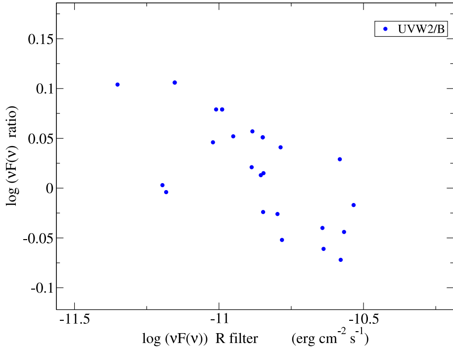
Fig. 12.— The ratio of \nu F(\nu) in the UVOT UVW2 filter to \nu F(\nu) in the UVOT B filter, as a function of \nu F(\nu) in the optical R filter.
