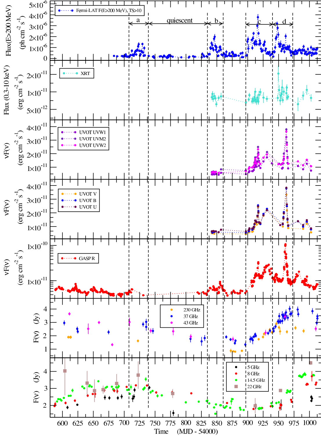
Fig. 7.— The MW light curves, from 2008 April to 2009 June. The vertical dashed lines show the four flaring episodes and the quiescent state.
