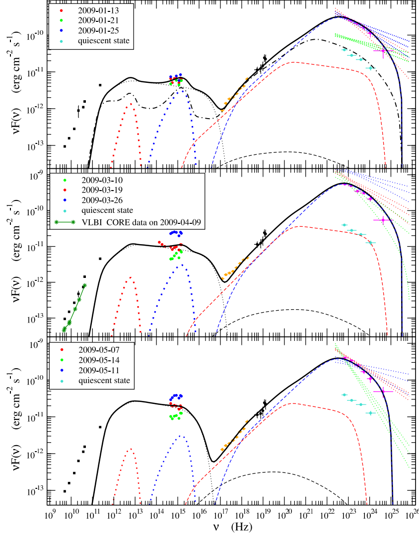
Fig. 24.— Red solid circles correspond to simultaneous Optical/UV data representing the intermediate state during the \gamma -ray integration period. Blue and green circles correspond to the highest and lowest flux state, respectively, observed during the same integration period. The Swift - XRT data (orange points) are integrated during the same interval of the LAT data, and the Swift - BAT data represent the 5-year fluxes discussed in Sect. 4.1. The black squares represent GASP radio data, integrated during the flares. The cyan points correspond to the LAT quiescent state SED. The magenta points represent the \gamma -ray SED integrated during the flare. The blue, green, and red dotted lines represent the PL best fit of the \gamma -ray data, for a daily integration and simultaneous to the Optical/UV data with the same color. The thin black dotted line represents the flaring synchrotron emission. The thin black dashed line corresponds to flaring SSC emission. The red and blue thick dotted lines correspond to the dusty torus and BBB emission respectively. The red and blue thin dashed lines correspond to the ERC/DT and ERC/BLR flaring emission respectively. The solid black thick line represents the sum of all the flaring model components. The thick dot-dashed line represents the sum of all the model components for the quiescent state alone.
