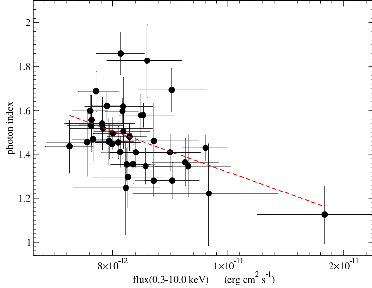
Fig. 8.— Scatter plot of the flux in 0.3 – 10.0 keV range vs. the X-ray photon index ( \alpha_X ). The dashed lines represent a linear bet fit model. Using the Monte Carlo method described in Sect. 2.2.1, we get a correlation coefficient r = -0.31 with a 95% confidence limit of -0.55 \leq r \leq -0.05
