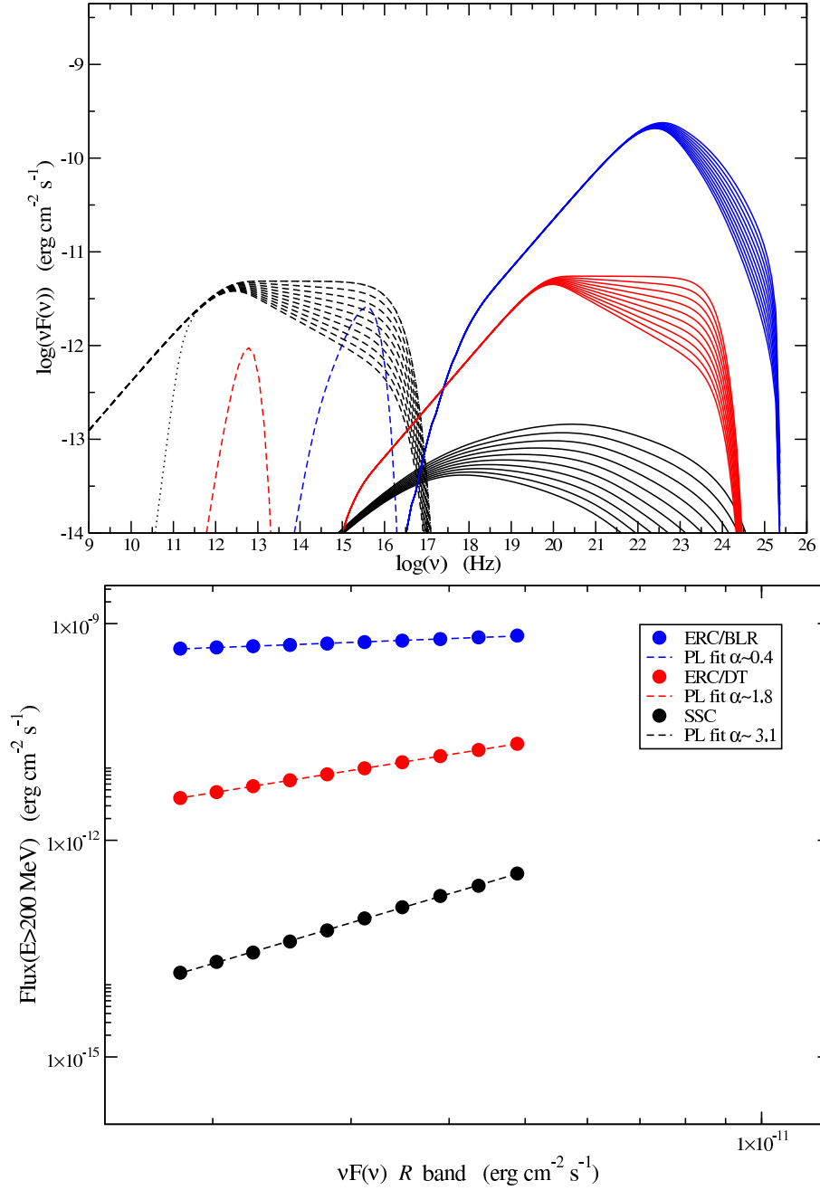
Fig. 25.— Upper Panel: the SEDs for the different values of the high energy electron distribution index. The black dashed lines represent the synchrotron emission without self absorption. The black dotted line represents the synchrotron self adsorbed emission. The black solid lines correspond to SSC emission. The red and blue dotted lines correspond to the dusty torus and BBB emission respectively. The red and blue solid lines correspond to the ERC/DT and ERC/BLR emission respectively. Lower Panel: optical/ \gamma -ray flux correlations for ERC/BLR (blue solid circles), ERC/DT (red solid circles), and SSC (black solid circles); dashed lines are the power law relations.
