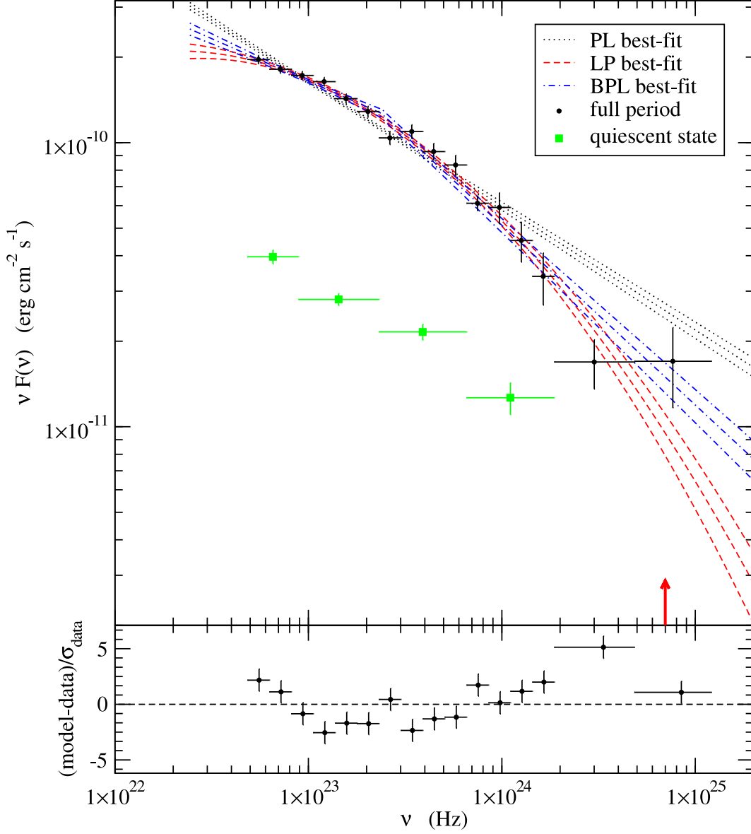
Fig. 3.— LAT SED of PKS 1510-089 extracted for the full period (black points) and for the quiescent state (green points). The red upward arrow indicates the highest energy event within 95% of the PSF for the whole period data set. The dotted line, the dashed line, and the dot-dashed line, represent the best fit model of the full period by means of PL, LP, a BPL distribution respectively, with uncertainties. The residuals in the lower panel refers to the PL model.
