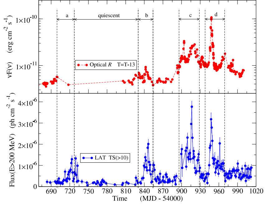
Fig. 18.— Upper Panel: the optical ( R ) light curve, obtained shifting the time according to the 13 days \gamma -ray lag reported in Sect. 4.2. Lower Panel: The Fermi -LAT light curve
