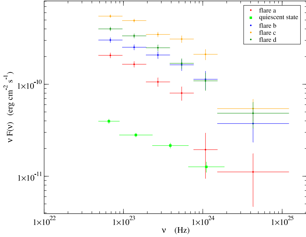
Fig. 4.— LAT SED of PKS 1510-089 extracted for the flaring states and for the quiescent state (green points).
