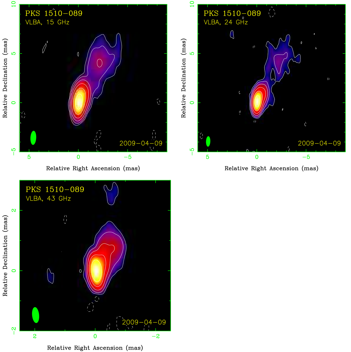
Fig. 21.— Stokes I CLEAN images of PKS 1510-089 observed by VLBA on 2009 April 9, at 15, 24, and 43 GHz. The lowest contour and peak intensity are 0.7 mJy/beam and 1.47 Jy/beam (15 GHz), 0.7 mJy/beam and 1.56 Jy/beam (24 GHz), 2 mJy/beam and 1.85 Jy/beam (43 GHz). Contours are plotted with a step \times 4 . Natural weighting of visibility data is used, HPBW beam size is shown in the lower left corner. Angular size of 1 mas corresponds to 5 pc.
