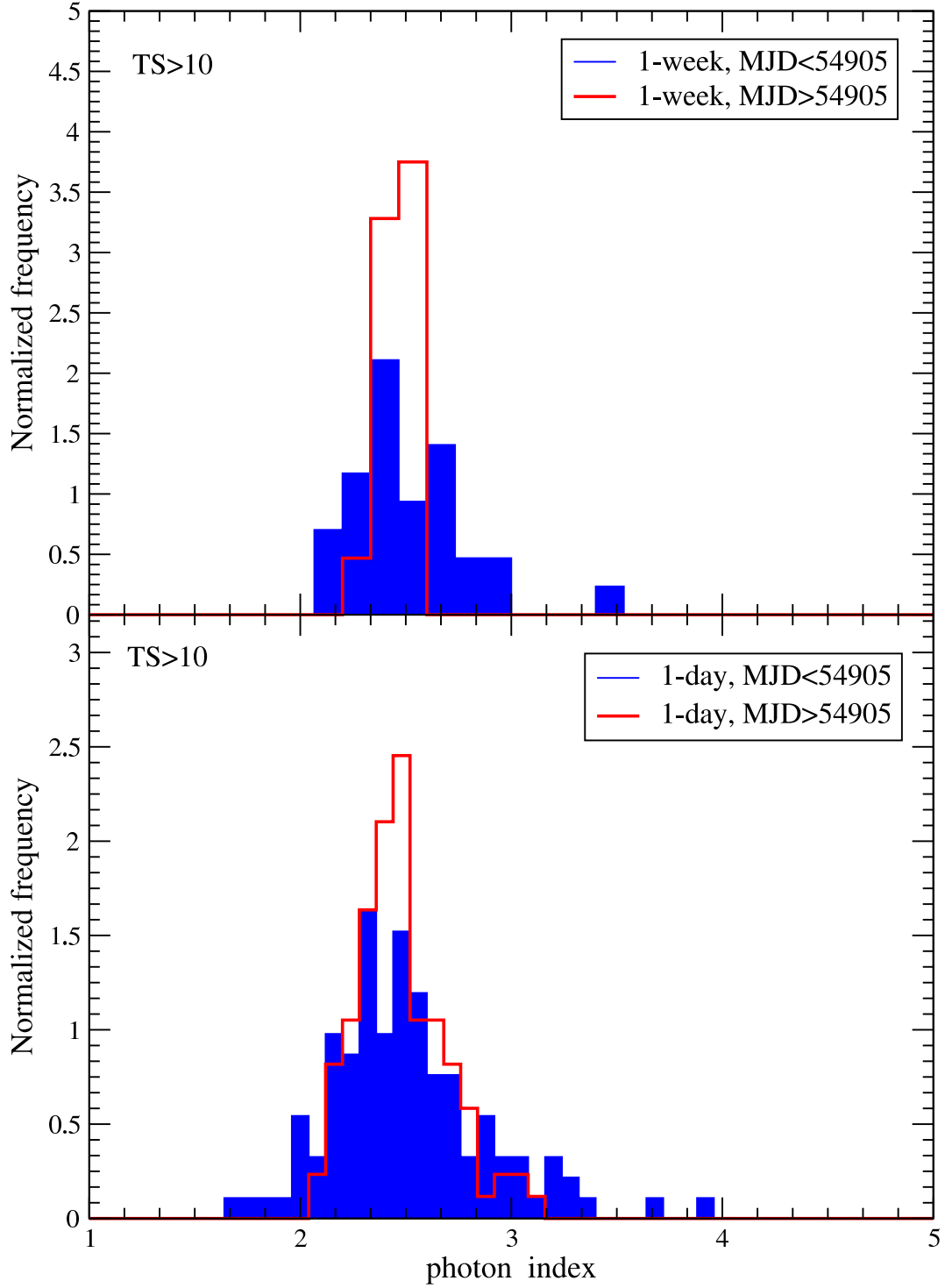
Fig. 6.— Upper Panel: The histogram of the photon index for, a weekly integration time, before (blue) and after (red) MJD 54905, respectively. Lower Panel: The same as in the upper panel, in the case of daily integration.
