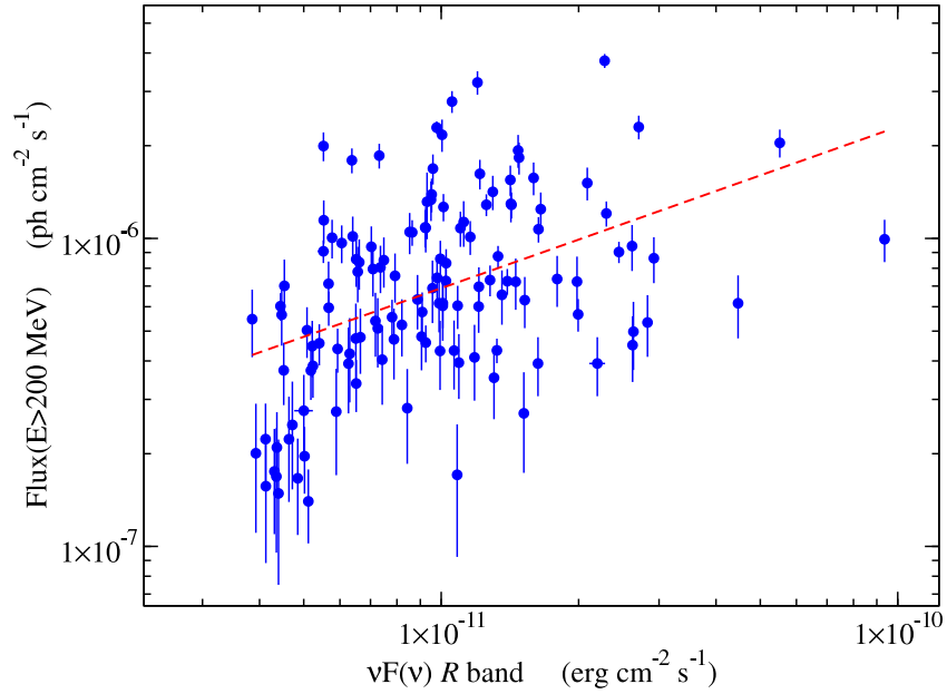
Fig. 16.— Scatter plot of the Fermi -LAT flux( E > 200 MeV) vs the \nu F(\nu) in the optical R band. The dashed line represents the best fit power-law model. The correlation coefficient of the logarithm of the optical and \gamma -ray fluxes, evaluated through the Monte Carlo method described in Sect. 2.2.1, is r = 0.42 with a 95% confidence interval 0.36 \leq r \leq 0.46 . There is an evident dispersion in the scatter plot, probably due to the inter-band time lags showed in Sect. 4.2
