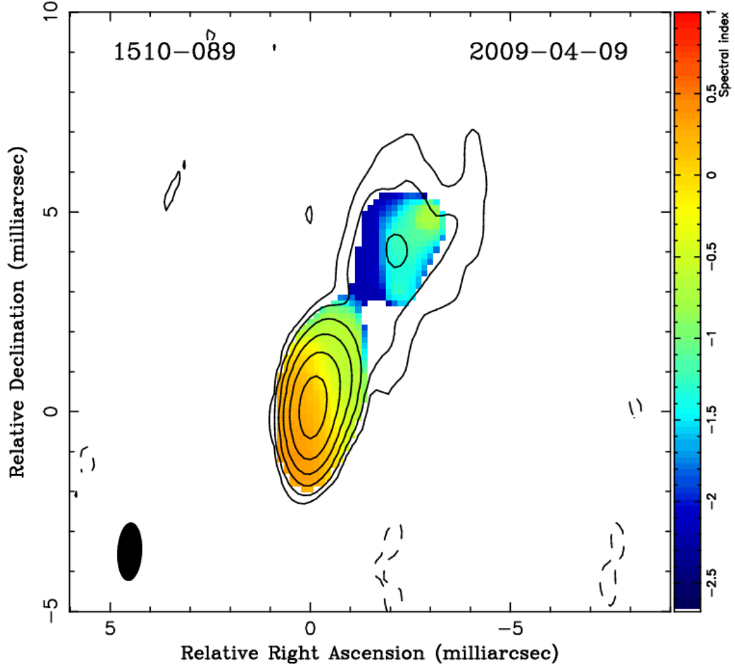
Fig. 22.— Spectral index s_r ( F(\nu) \propto \nu^{s_r} ) map between 15.4 and 23.8 GHz (shown in color) of PKS 1510-089 as observed by the VLBA on 2009 April 9. The overlaid contours represent total intensity at 15.4 GHz (see Figure 21 for details). The spectral index map was smoothed by a median filter with a 0.6 mas radius.
