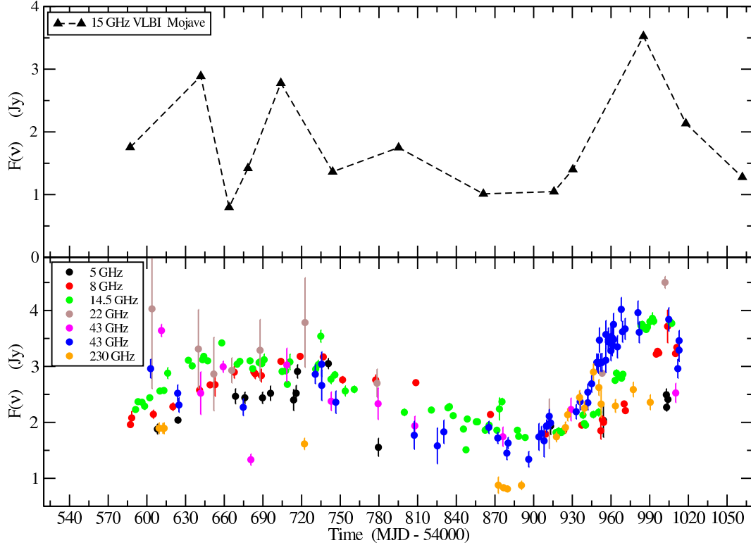
Fig. 20.— Upper panel: The 15 GHz MOJAVE VLBA parsec-scale core light curve. Lower panel: GASP radio light curve.
