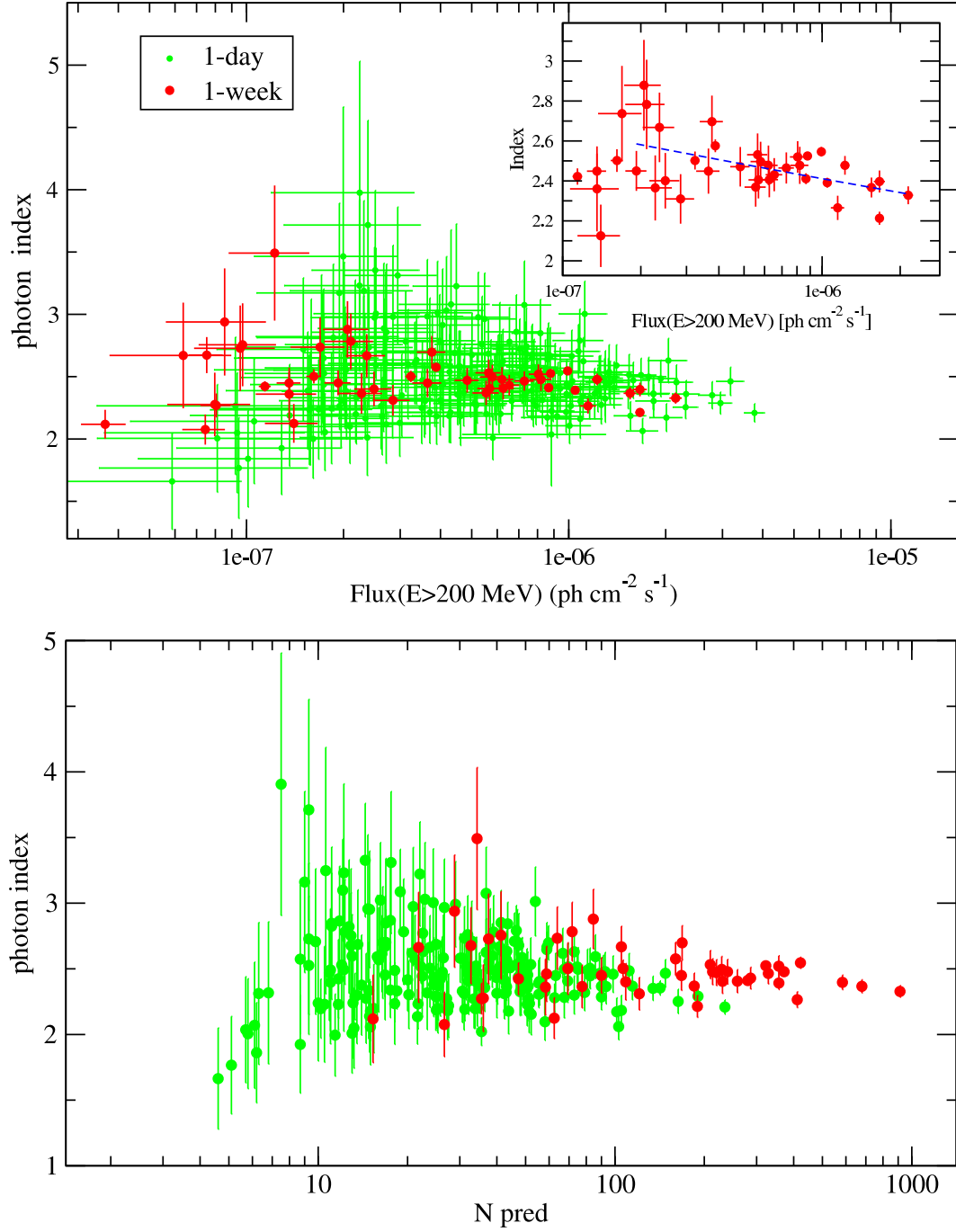
Fig. 5.— Upper Panel: weekly and daily scatter plot of the Flux( E > 200 MeV) vs. the photon index (TS > 10). The inset shows the same for Flux( E > 200 MeV) > 2 \times 10^{-7} \text{ ph cm}^{-2} \text{s}^{-1} . Lower Panel: Scatter plot of the number of photons predicted by the best-fit model vs. the photon index, for weekly and daily integration (TS > 10).
