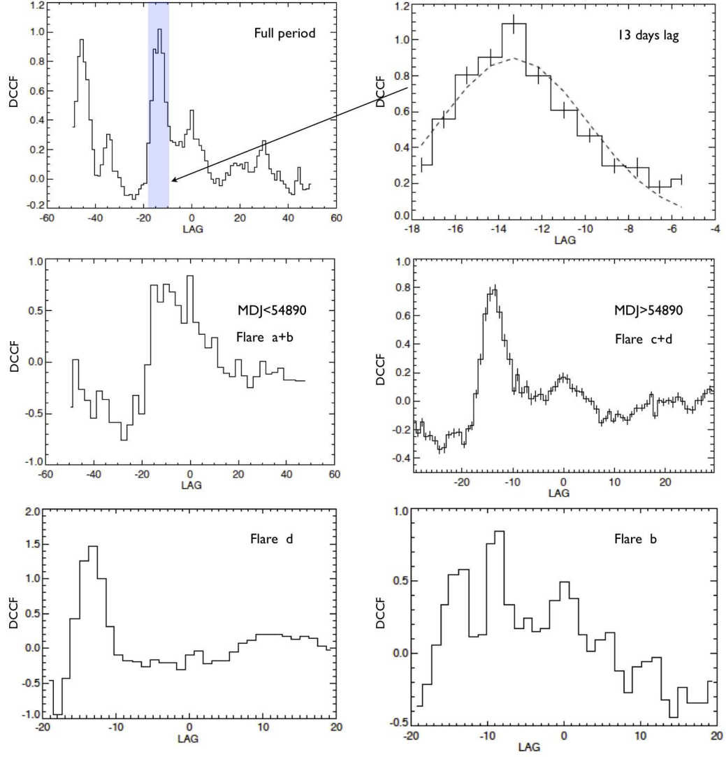
Fig. 17.— Top panel, left: DCCF for the whole analysis period, the shaded box concerns the 13 days lag. Top panel, right: fit by means of Gaussian distribution of the 13 day lag shaded in the left panel, the fit returns a lag of -13.4 \pm 0.2 , gamma leading optical. Middle panels: the DCCF for MDJ<54890 (left panel) and MDJ>54890 (right panel). The lag of about 13 days with the \gamma -ray leading the optical band is still there. Bottom panels: a lag of about 13 days (gamma leading optical) is also present for flare d and b individually.
