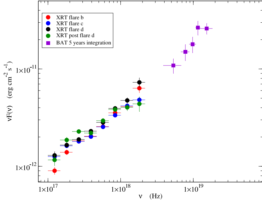
Fig. 9.— XRT SEDs averaged during the flare b , c , d and duiring the post d flare period. The violet boxes represent the BAT spectrum averaged over 5 years
