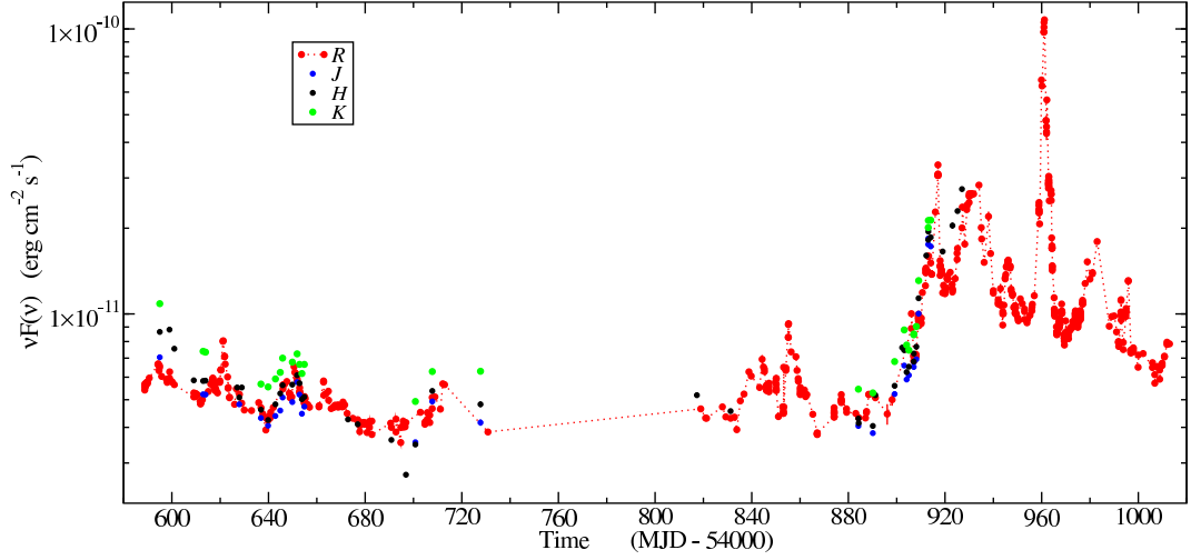
Fig. 15.— Optical and near-IR light curves from the GASP project.
