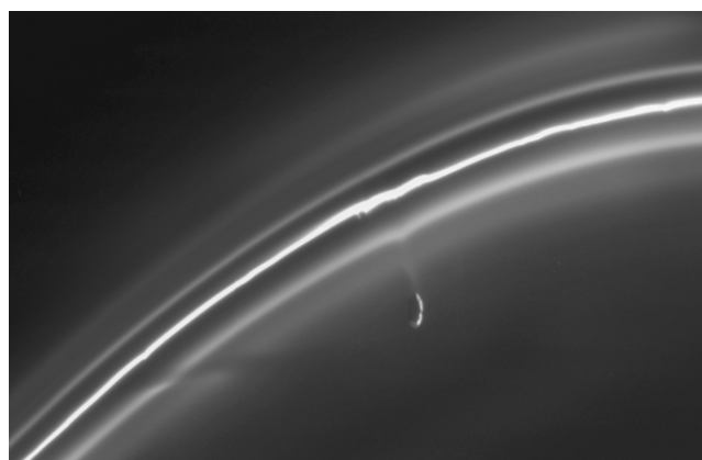
Figure 3.10 Image of the multi-stranded F ring and the nearby 135-km (long axis) ring-moon Prometheus, having a close encounter with the ring. The main core is the brightest, central ringlet, which has maintained a stable, precessing Keplerian orbit for over three decades. The outlying fainter strands are transitory features, resulting from the wrapping up into tight spirals of large jets of ejecta created by rare, sizeable objects (still much smaller than Prometheus) crashing through the F Ring core (Charnoz et al. , 2005). The faint, nearly horizontal feature crossing the strands at bottom left is a “gore” created by Prometheus perturbations on a prior close encounter with this patch of material (Murray et al. , 2008, see also Chapter 13). Image PIA 06143; courtesy NASA/JPL and SSI.
