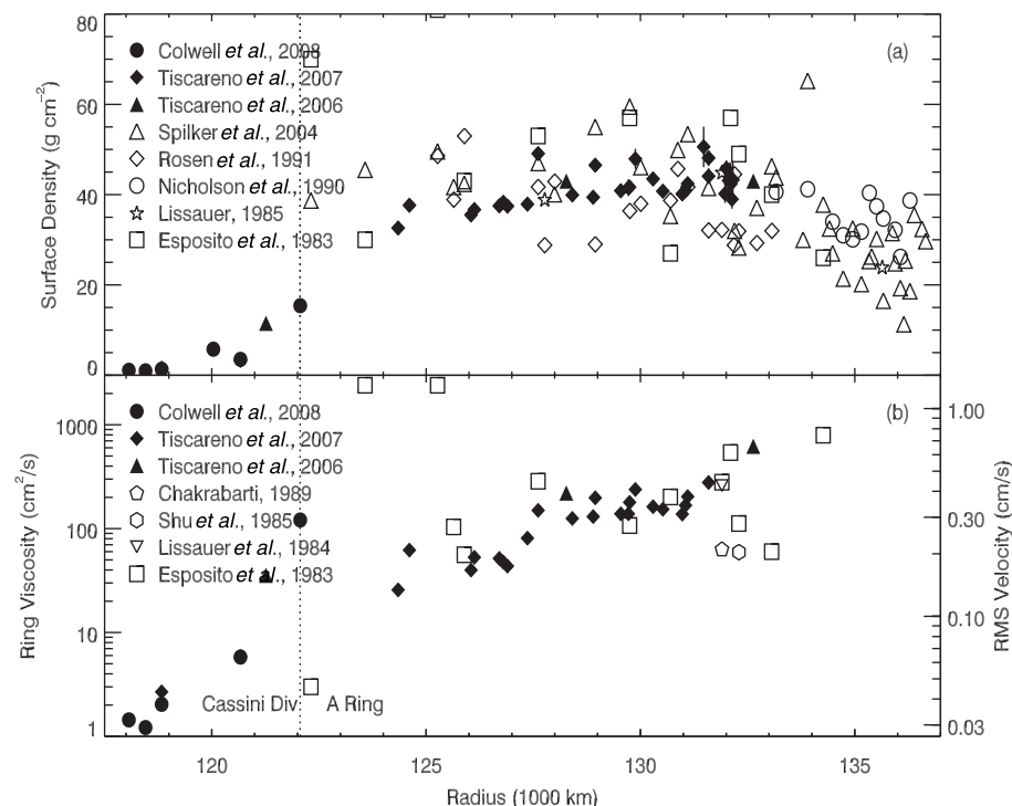
Figure 3.6 A collection of determinations of surface mass density from density wave wavelengths, and viscosity from wave damping lengths. Cassini results are shown in filled symbols, and Voyager results in open symbols. The vertical dotted line is the inner edge of the A ring (figure from Colwell et al. , 2009, where references are given).
