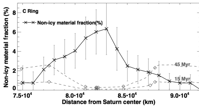
Figure 3.19 Black curve: Non-icy material fraction derived from Cassini 2 cm radiometer observations. Gray dashed curve: The non-icy material fraction as evolved over 15 and 45 Myr if meteoroid bombardment is the only source of contamination in a structurally fixed ring, and the flux has remained constant. Gray diamonds indicate locations where opacity measurements have been made through density waves. Figure adapted from Zhang et al. (2017).
