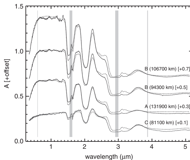
Figure 3.24 Spectral fit of the Bond albedo A for four ring regions, C(81100 km), B(94300 km), B(106700 km), A(131900 km) adapted from Ciarniello et al. (2016). The solid curves are the Bond albedo retrieved from VIMS observations and dotted lines the modeled spectra. Vertical gray bars correspond to VIMS order sorting filter junctions. Spectral modeling compositional parameters are given in Table 3.1.
