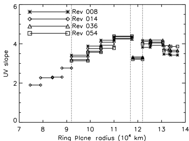
Figure 3.18 The spectral slope calculated as the ratio of I/F between 175 and 190 nm (just longward of the water ice absorption edge) to that between 140 and 160 nm (shortward of the ice edge), so in some sense a metric for the fractional abundance of uncontaminated water ice (Bradley et al. , 2010). Note, however, that the radial profile is qualitatively different from the radial profile of water ice band depth (curves C and D in Figure 3.15). A more noticeable step near 10^5 km, consistent with Figure 3.15, would be inferred from ratioing the two A_B profiles in Figure 3.17.
