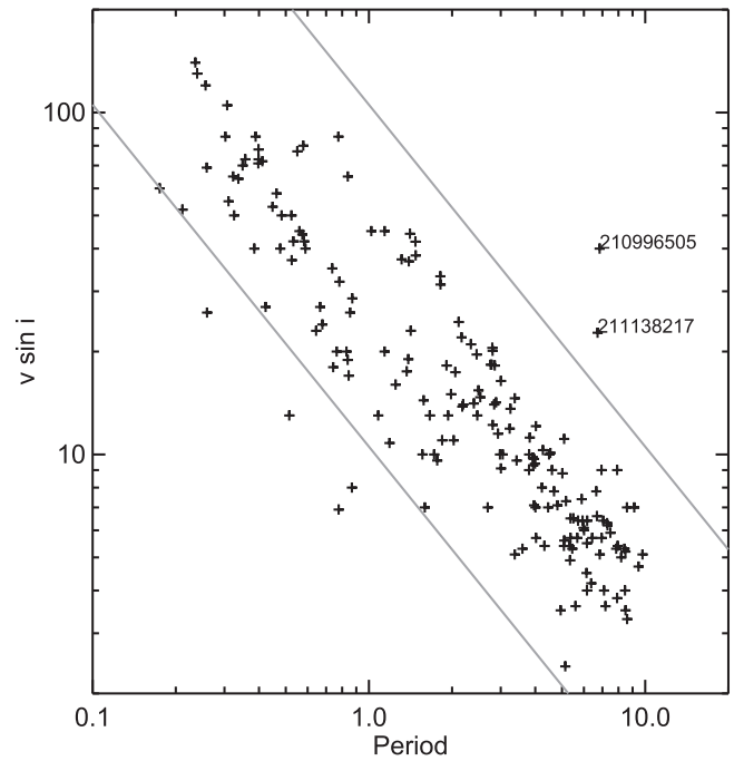
Figure 6. P (in days) vs. v \sin i (in \text{km s}^{-1} ) for stars in this study for which there are v \sin i values in the literature. The gray lines correspond to the expected relationship between P and v \sin i ( = (2\pi R \sin i)/P ) for i = 90^\circ and 6^\circ , assuming R = 0.5 R_\odot . The P and v \sin i agree well, except for two cases—both of which are earlier-type stars with a secondary component, where the v \sin i is probably from the primary and the P is from the lower-mass secondary. They are EPIC 210996505/HII1132 and 211138217/HII1766.
