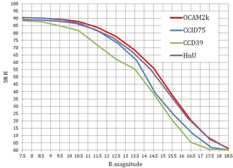
Figure 2: the SOUL improvement in the LBT AO performance (the current is in green line) with different CCD choices, computed with a seeing of 0.8"
