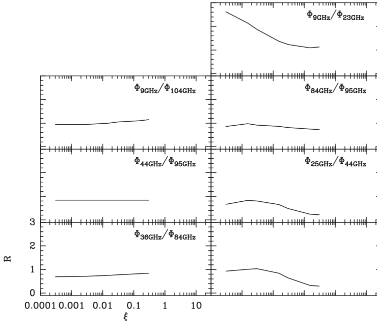
Figure 2. Modelled ratios between photon production rates of several CIMMs for T = 200\text{ K} and a volume density n = 10^7\text{ cm}^{-3} . In the left panel, we show ratios among transitions within same families, while in the right panel we plot ratios among CIMMs from different families.
