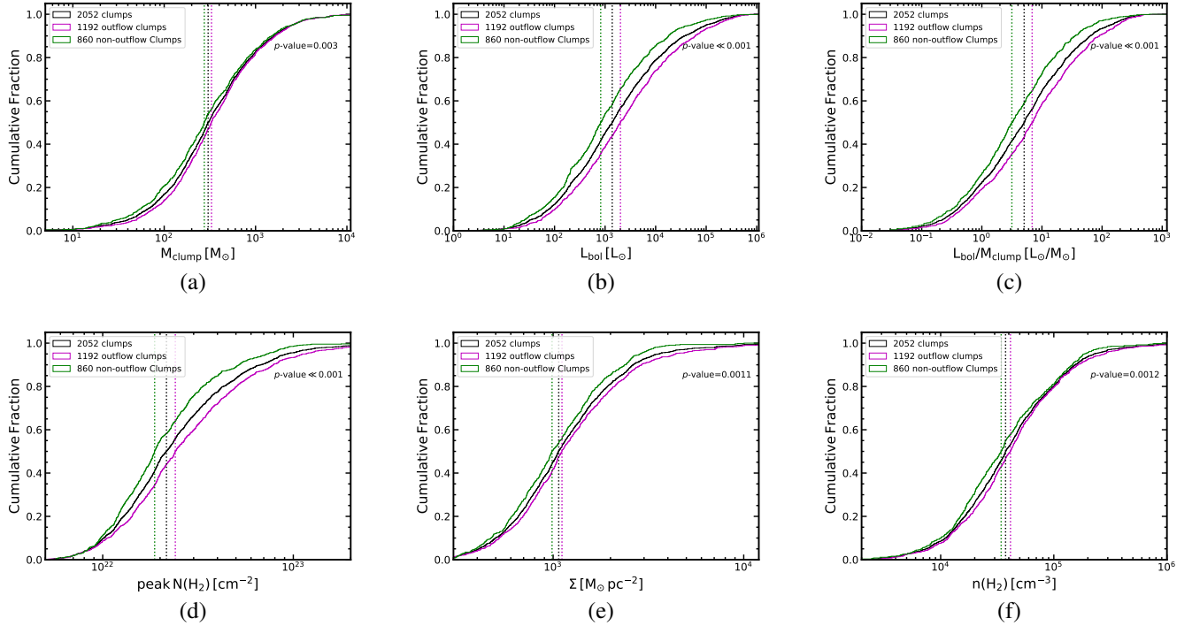
Fig. 4. Cumulative distributions of the physical properties for the total 2052 clumps, the 1192 outflow clumps, and the 860 non-outflow clumps. Top left (a,b,c) to bottom right (d,e,f): cumulative distributions of clump mass ( M_{\text{clump}} (M_{\odot}) ), bolometric luminosity of central objects ( L_{\text{bol}}/L_{\odot} ), luminosity-to-mass ratio ( L_{\text{bol}}/M_{\text{clump}} (L_{\odot}/M_{\odot}) ), the peak \text{H}_2 column density ( \text{peak } N(\text{H}_2) \text{ cm}^{-2} ), the mean mass surface density ( \Sigma (M_{\odot} \text{ pc}^{-2}) ), and the mean volume \text{H}_2 density ( n(\text{H}_2) (\text{cm}^{-3}) ) of the total 2052 clumps (black lines), the 1192 outflow clumps (magenta lines), and the 860 non-outflow clumps (green lines). We present the median values of the three samples in vertical lines, and p -values of K-S tests between the outflow sample and the non-outflow in each plot.
