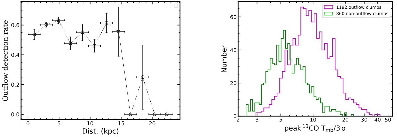
Fig. 7. Distribution of the ratio between the peak intensity of the 13 CO line and the 3σ detection level of the corresponding spectrum for the outflow sample (magenta histogram) and the non-outflow sample (green histogram).
