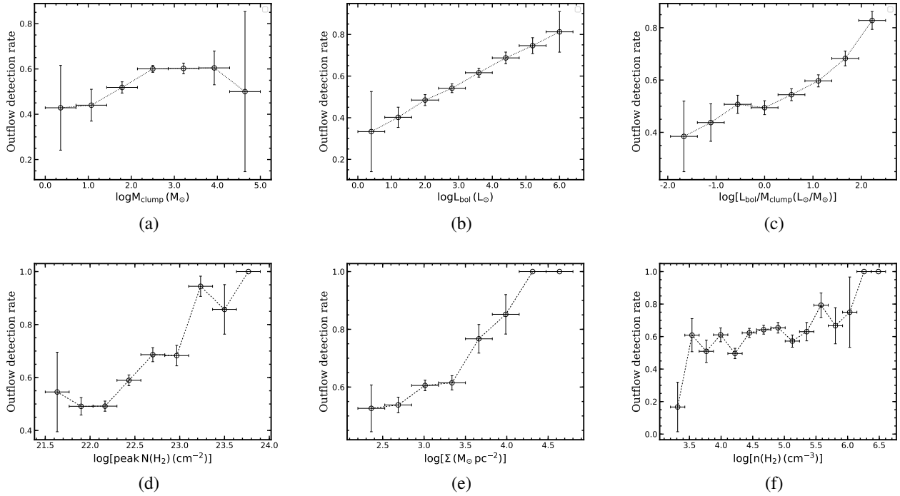
Fig. 9. Outflow detection rate against the physical properties of clumps. Top left (a,b,c) to bottom right (d,e,f): detection rate as a function of clump mass M_{\text{clump}} ( M_{\odot} ), bolometric luminosity of the central object L_{\text{bol}}/L_{\odot} , luminosity-to-mass ratio L_{\text{bol}}/M_{\text{clump}} ( L_{\odot}/M_{\odot} ), the peak \text{H}_2 column density (peak N(\text{H}_2) \text{ cm}^{-2} ), the mean mass surface density \Sigma ( M_{\odot} \text{ pc}^{-2} ), and the mean volume \text{H}_2 density n(\text{H}_2) ( \text{cm}^{-3} ) of clumps in logarithmic scales. The error bars on the x -axis and y -axis are determined following the same method in Fig. 6.
