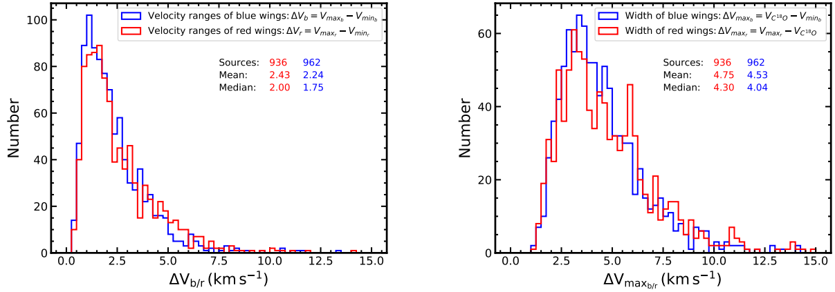
Fig. 5. Distributions of velocity ranges \Delta V_{b/r} (left panel), maximum blue and red wing velocities \Delta V_{\max b/r} (right panel) of the 1192 clumps with outflow wings, including 706 clumps with bipolar wings, and 486 clumps with unipolar wings.
