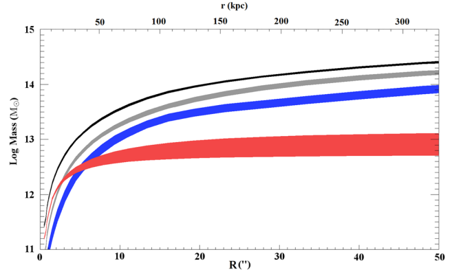
Figure 6. Projected 2D mass profile at 68 per cent confidence level of the core of MACS 2129 . In red, we plot the BCG stellar mass profile, in blue we plot the total mass of the other cluster members, in grey the cluster DH and in black the total mass profile.
