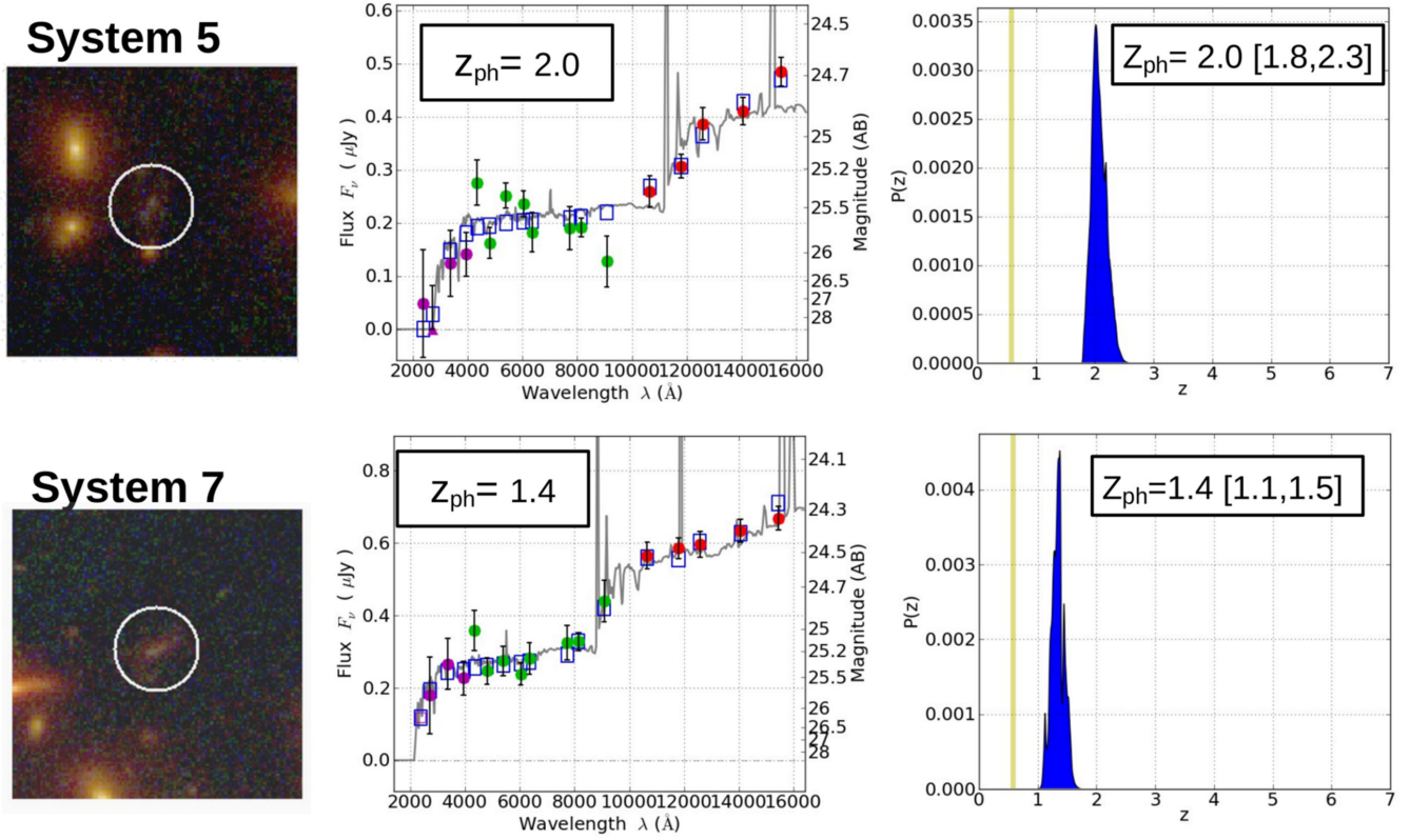
Figure A3. SED for the multiple images systems 5 and 7, derived using the CLASH photometry and the SED fit code BPZ. We present the fit of the multiple images 5.2 and 7.3, which get well-defined \text{PDF}(z) . On the left, we show the lensed images cut-out in the colour composite image of the cluster. The white circle labels the image and has diameter of \sim 1.5 arcsec. The central panel shows the SED fitted with the photometric measurement from CLASH, showing in violet the fluxes in the WFC3UVIS filter, in green the one in the ACS and in red the IR photometry observed with the WFC3IR. The grey line shows the best template fitting the photometry, and in the legend we provide the respective best-fitting redshift. On the right, we show the respective \text{PDF}(z) and provide the best-fitting z_{\text{ph}} with the respective 68 per cent confidence level interval. The vertical yellow line marks the cluster redshift.
