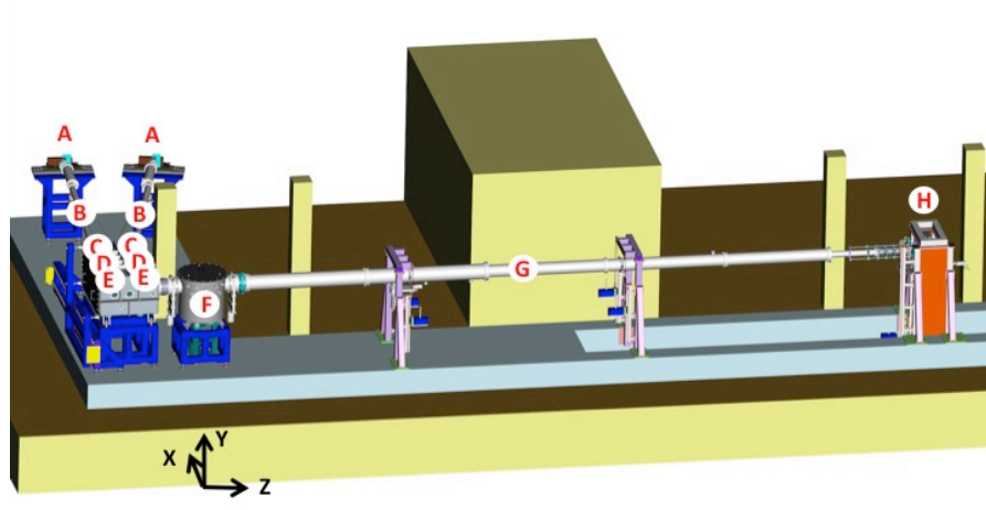
Figure 2. Mechanical design of the vacuum system, showing the optical components and the coordinate system
