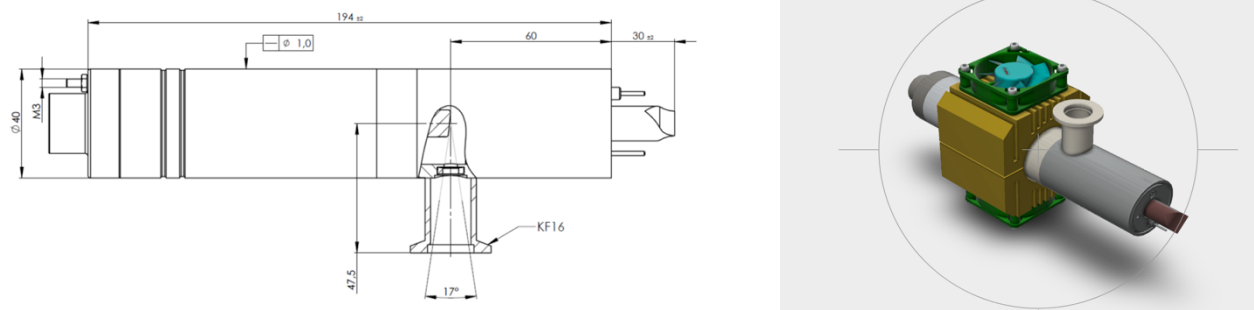
Figure 3: Left: Design sketch of the tube. Right: CAD model of the Ti microfocused tube, showing the forced air cooling system (credits Incoatec)
