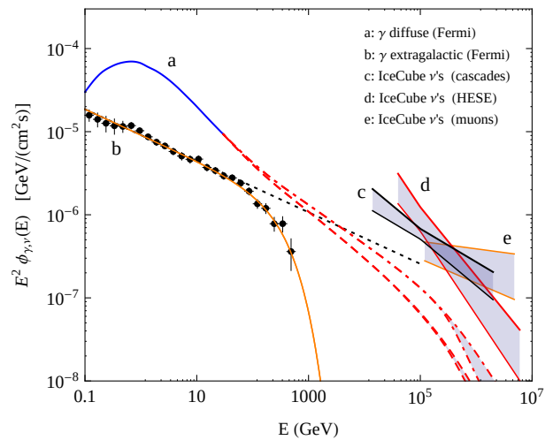
FIG. 16: Curve a shows the diffuse Galactic gamma ray flux observed by Fermi (solid line) and the extrapolations calculated under the assumptions of a factorized (dashed line) and non-factorized (dot-dashed line) emission. The Fermi measurement of the extragalactic gamma ray flux [55] is shown by as line b (and with the points). The shaded regions c d and e show estimates of the neutrino flux obtained by IceCube under the assumption of an isotropic extragalactic flux [17]. All fluxes are integrated over the entire sky.
