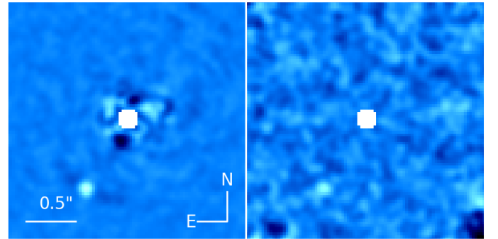
Fig. 1. Final PSF-subtracted images from the two NACO datasets in L' (left panel) and M' (right panel). The companion is detected in both datasets. While we find a lower contrast ratio in M' , the high thermal background leads to a lower overall SNR.
