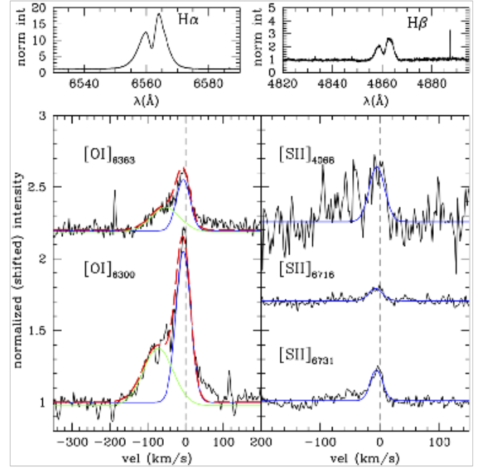
Fig. 5. FEROS spectrum of RCrA. Top panels: regions around H \alpha and H \beta lines. Bottom panels: regions around [O I] \lambda 8446 and [S II] \lambda 4068/6716/6731 forbidden lines. The colored Gaussian profiles in the bottom panels refer to the multiple component deconvolution: in green, the HVC, in blue, the LVC, in red, the sum of the two components.
