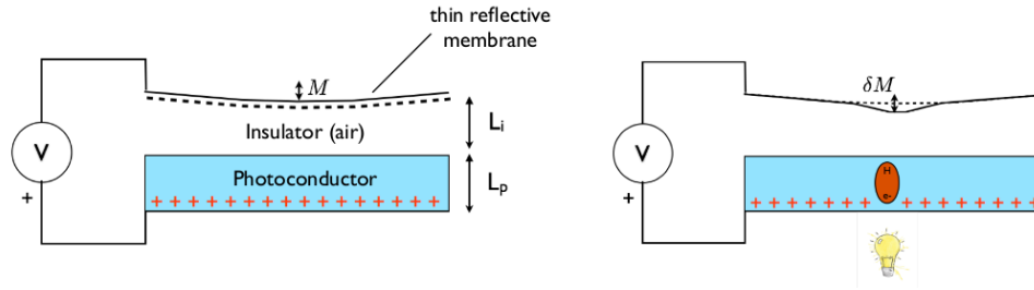
Fig. 1. PCDMs functioning scheme in DC: a) before illumination, b) after illumination.
