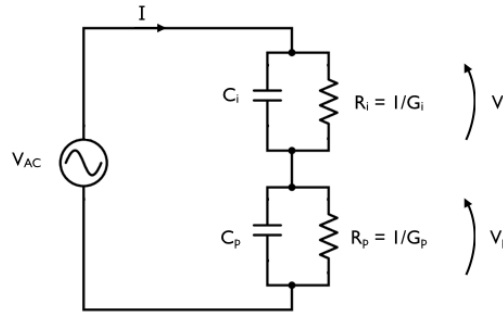
Fig. 2. PCDMs electrical model.
