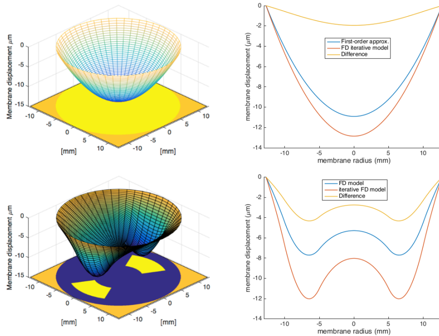
Fig. 5. Examples of a 1" diameter ZnSe-based PCDM response to the light patterns depicted at the bottom of the plots on the left. Blue zones: no light, yellow zones: 10 \text{ mW/cm}^2 , orange zones: outside the PCDM region. The comparison between approximated model of [8, 13], finite difference (FD) model and our iterative FD model is shown in the sections on the right. Simulations were run with the following parameters: 200 V_{PP} , 100 Hz, ZnSe thickness 3 mm, membrane-photoconductor distance 50 \text{ }\mu\text{m} , membrane tension 50 N/m.
