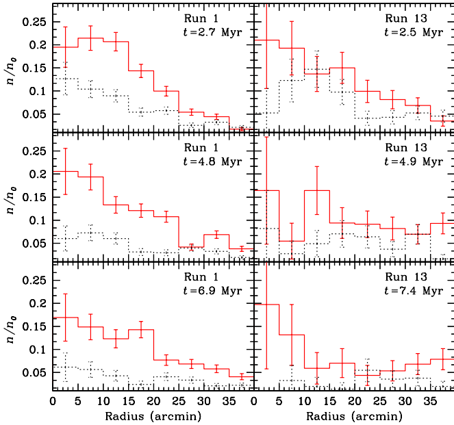
Fig. 4. Normalized radial stellar density in run 1 (left-hand panels) and in run 13 (right-hand panels) at different times. The simulated cluster is assumed to be at a distance of 350 pc. Solid red line: pop. A; dotted black line: pop. B. The density n is calculated as stars per arcmin 2 , within concentric annuli. The normalization n_0 was chosen so that the total area below the histogram of pop. A is one. The error bars account for Poisson uncertainties.
