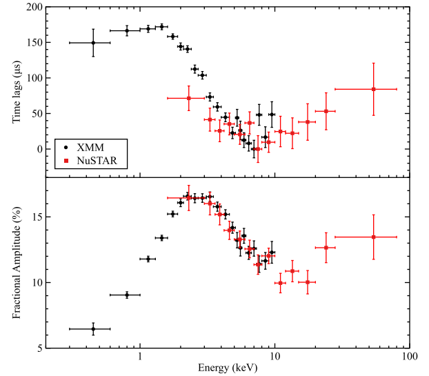
Figure 4. Top panel: time lags in \mu s evolution as a function of energy obtained from the XMM-Newton and NuSTAR observations reported with black dots and red squares, respectively. For display purpose only the reference pulse profiles of the two data sets have been set around 7 keV. Bottom panel: evolution of the pulse fractional amplitude for the two data sets. The colour coding has been kept fixed between the panels.
