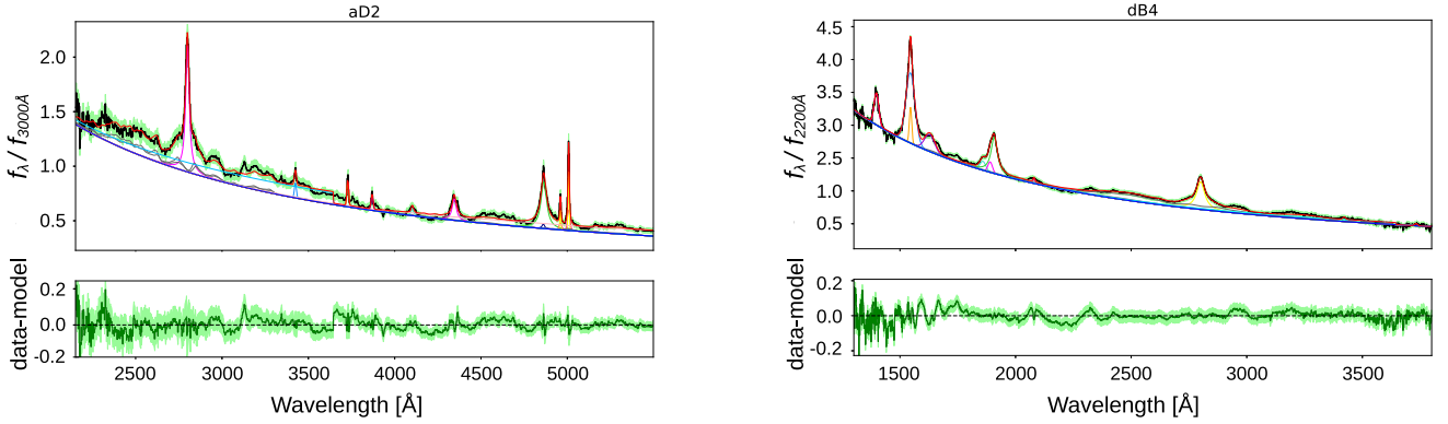
Fig. 2. Examples of a low-redshift bin (left) and a high-redshift bin (right) fit. The continuum power law is marked in blue, Fe II templates in grey, emission lines in different colours (orange, purple, green, cyan). The total model is depicted in red.
