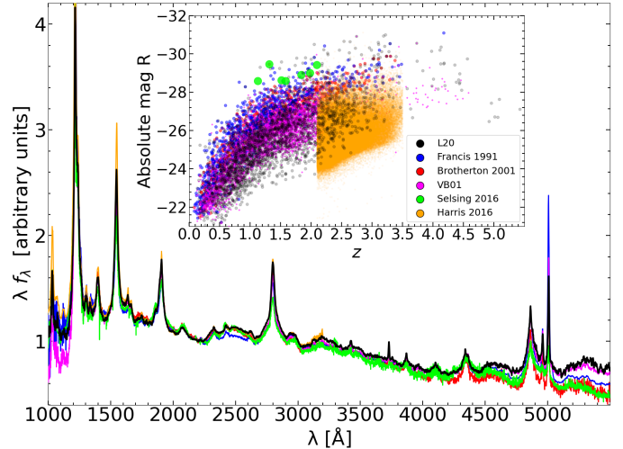
Fig. 4. Comparison between our quasar template and others from the literature. All the templates are scaled by their emission at 2200 Å. The agreement on the UV side, apart from minor differences in the Fe II pseudo-continuum, specifically the 2250–2650 Å and the 3090–3400 Å bumps, is apparent. The Ly \alpha emission line is cut for visualisation purposes. The inset shows the distribution of the absolute R magnitude against the redshift for the different samples reported.
