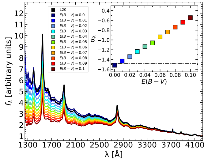
Fig. 11. Extinction of the VB01 template according to the colour-coded values. All the spectra are scaled by their 4200-Å flux, where extinction becomes less relevant. The black spectrum is our full sample stack and is in very good agreement with a low degree of extinction. The inset shows the best-fit slope in the range 1300–4100 Å of the VB01 template reddened as a function of the E(B - V) value. The black dot-dashed line represents the slope of the continuum fitted to our stack. Minimal levels of extinction are allowed to match the reddened template with our composite. We note that the visual match between the L20 and the VB01 reddened template depends slightly on the scaling wavelength. The slope derived from the fits, however, does not depend on such a wavelength.
