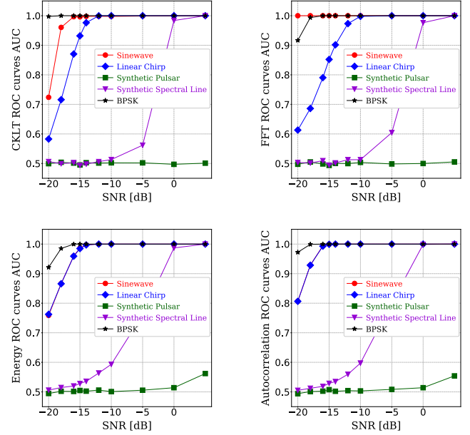
Figure 9. AUC as a function of the SNR of the ROC curves for the CKLT detector (top-left panel), the FFT detector (top-right panel), the energy detector (bottom-left panel), and the autocorrelation detector (bottom-right panel).
