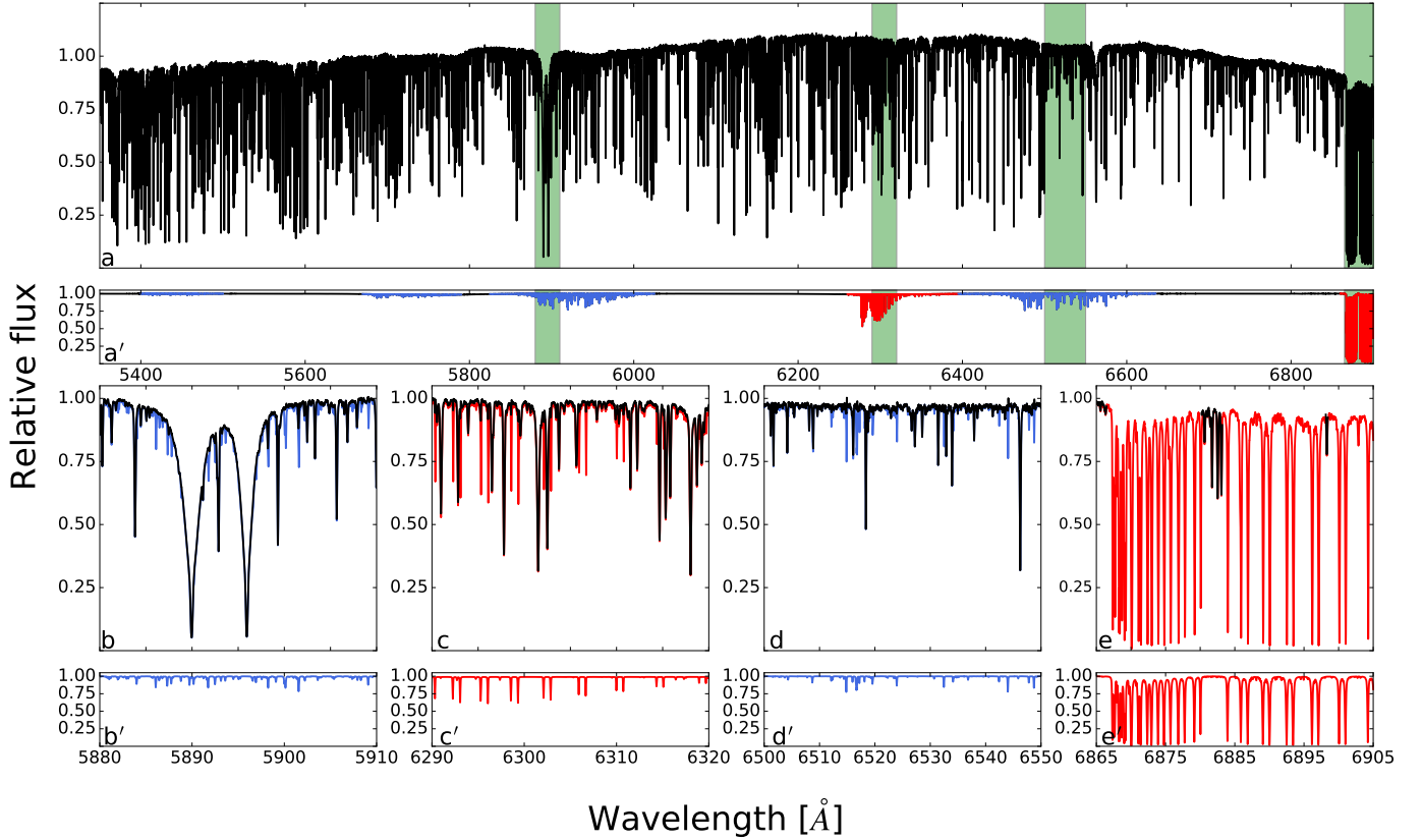
Fig. 1. Influence of telluric lines on the spectrum of HD 189733 obtained with HARPS on the red part of the CCD (5380 to 6900 Å) for the night of 19 July 2007. The upper panel a–e is the observed stellar spectrum with telluric contamination. Panel a'–e' is the best fit telluric model obtained with Molecfit with H 2 O in blue and O 2 in red. Panels b, b'; c, c'; d, d'; and e, e' are close-up views of the green zones in panel a, a' . These contain the strongest telluric bands in the visible (from left to right: H 2 O (203-000, 302-000, 321-000) band at ~5900 Å around the Na doublet, O 2 γ band at ~6200 Å, H 2 O (311-000) band at ~6500 Å and O 2 B band at ~6900 Å).
