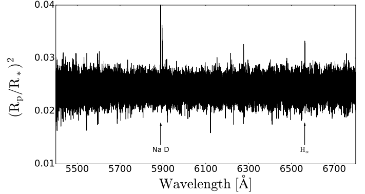
Fig. 3. The combined transmission spectrum of HD 189733b. The Na doublet is visible at \sim 5890 \text{ Å} and the H- \alpha line at 6562 \text{ Å} .
