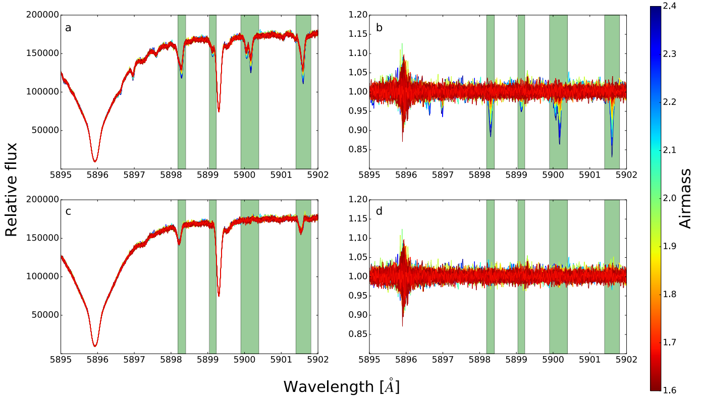
Fig. 2. Variability in the spectra over the night of 19 July 2007 for some water lines in the band at 5900 Å with the Na I D1 line on the left. The colorbar indicates the airmass. Panel a shows the non-corrected spectra. Green bands indicate the strongest telluric lines. Panel b is the variation of each non-corrected spectrum from the mean spectrum of the night. Panel c shows spectra corrected from the telluric lines using Molecfit. Panel d is the variation of each corrected spectrum from the mean spectrum.
