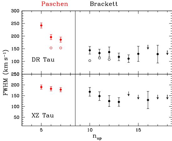
Fig. 9. Measured FWHM of H I Paschen and Brackett lines in DR Tau (upper) and XZ Tau (bottom). Upper limits are indicated by arrows. Open dots in the DR Tau plot indicate the width of the main line component once the blue-shifted component has been removed through profile decomposition.
