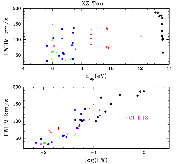
Fig. 10. FWHM of the permitted lines detected in XZ Tau plotted as a function of the log of the EW (bottom) and the energy (in eV) of the upper level (top). Symbols and colour-codes are as follows: black filled circles = H I; blue filled squares = Fe I; red filled triangles = C I; green open triangles = Si I; purple crosses = others.
