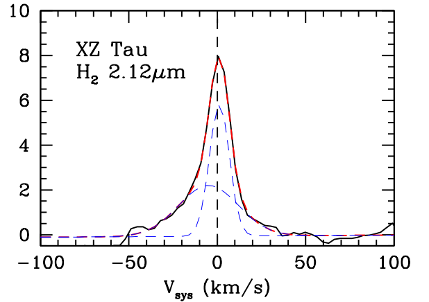
Fig. 13. Profile of the H 2 2.12 μm line detected in XZ Tau with the fit of the two Gaussian components superimposed. The red-dashed line is the best fit obtained by the sum of the two Gaussian components plotted as blue-dashed lines. Parameters of the two components are given in Table 2.
