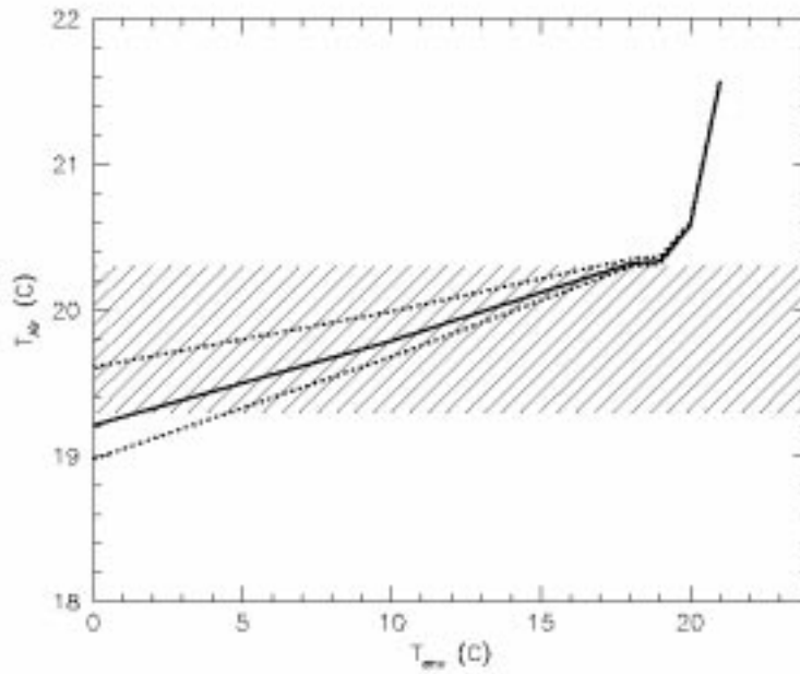
Fig. 8. Run of expected temperature of SARG as a function of temperature in the Nasmyth room when the DATCS is in operation. Solid line represents average (air) temperature; dotted lines are expected minimum and maximum temperatures within the spectrograph. The dashed area represents specifications.
