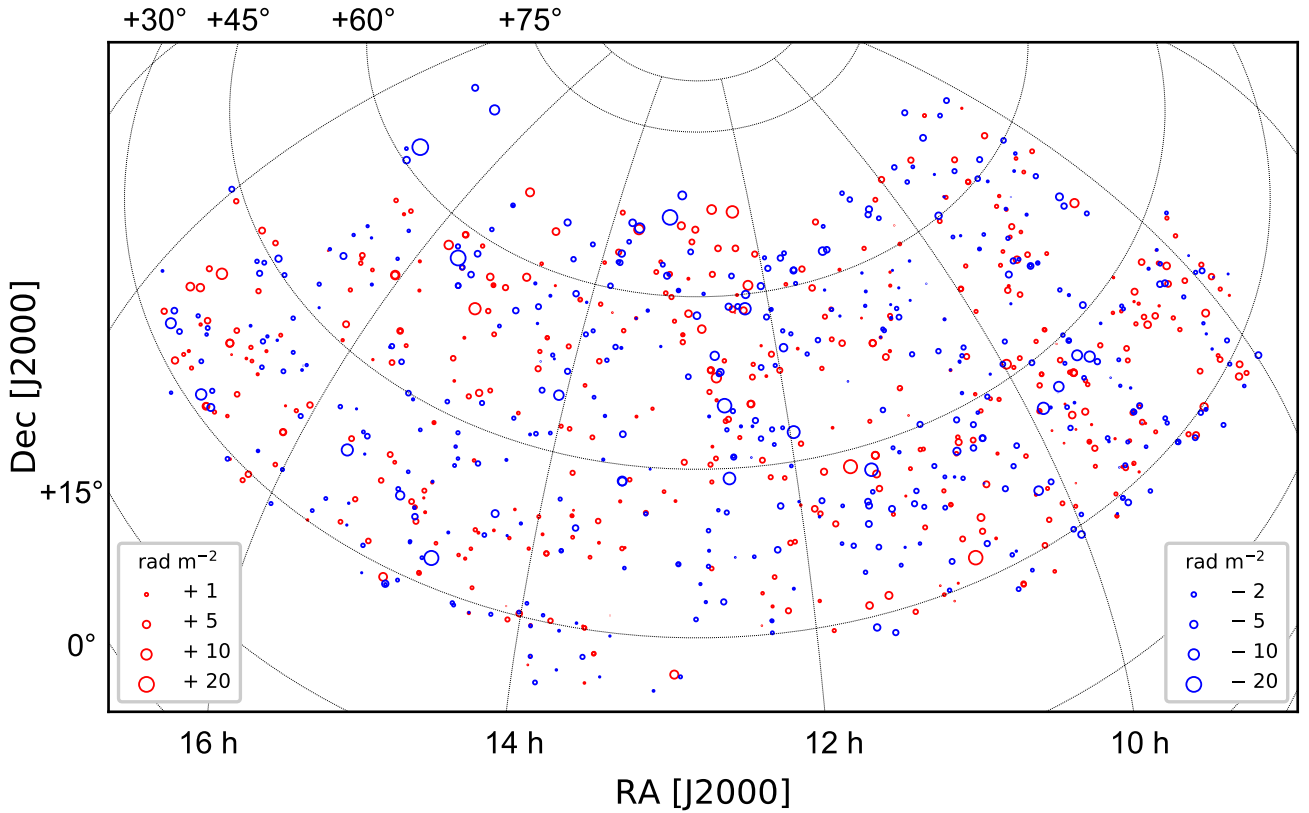
Figure 1. Sky distribution of the RRM sample used in the analysis. The field of the LoTSS DR2 survey centred at RA = 13h is shown.
