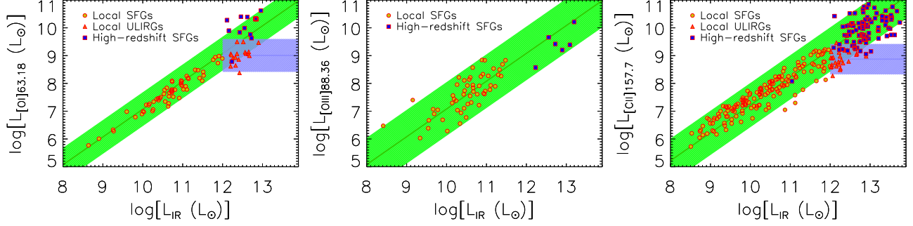
Figure 2. Luminosity of the [OI] 63.18 \mu\text{m} (left panel), [OIII] 88.36 \mu\text{m} (central panel) and [CII] 157.7 \mu\text{m} (right panel) lines, versus continuum IR luminosity. The green bands show the 2\sigma range around the mean relation \log(L_{\ell}/L_{\odot}) = \log(L_{\text{IR}}/L_{\odot}) + c for local SFGs with L_{\text{IR}} < 10^{12} L_{\odot} (yellow circles) and high-redshift SFGs (blue squares); the values of c \equiv \langle \log(L_{\ell}/L_{\text{IR}}) \rangle are given in Table 1. The azure bands show the 2\sigma spread around the mean line luminosity for the sample of local ULIRGs ( L_{\text{IR}} \geq 10^{12} L_{\odot} ; orange triangles) whose line luminosities appear to be uncorrelated with L_{\text{IR}} and are generally lower than expected from the linear relation holding for the other sources. The mean line luminosities \langle \log(L_{\ell}/L_{\odot}) \rangle of these objects are given in Table 1 as well. See text for the sources of data points.
