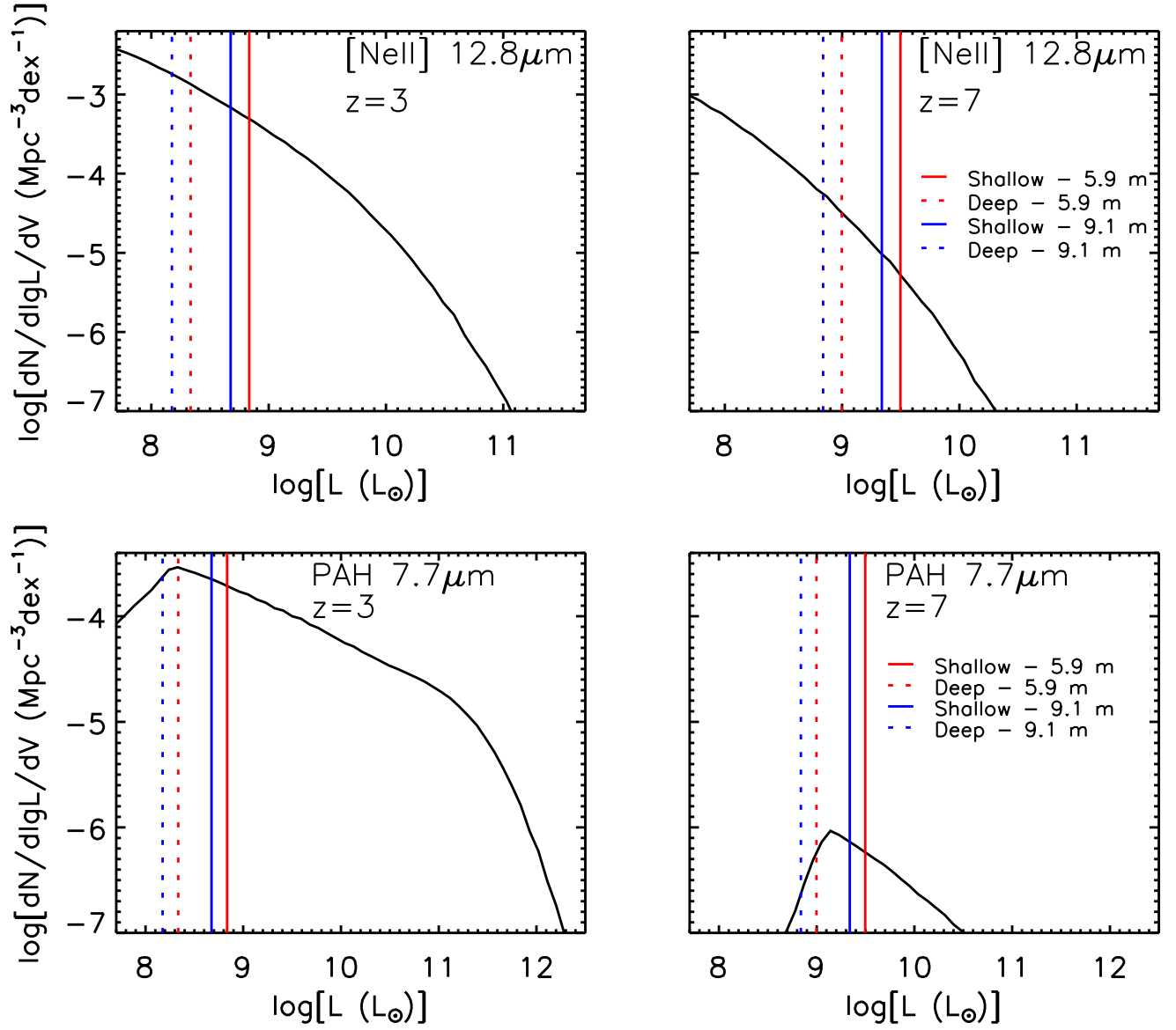
Figure 13. Luminosity functions of the fine structure line [\text{NeII}] 12.8 \mu\text{m} (upper panels) and the PAH 7.7 \mu\text{m} line at z = 3 and z = 7 . The decline of the faint end of the PAH luminosity function is due to the effect of decreasing metallicity.
