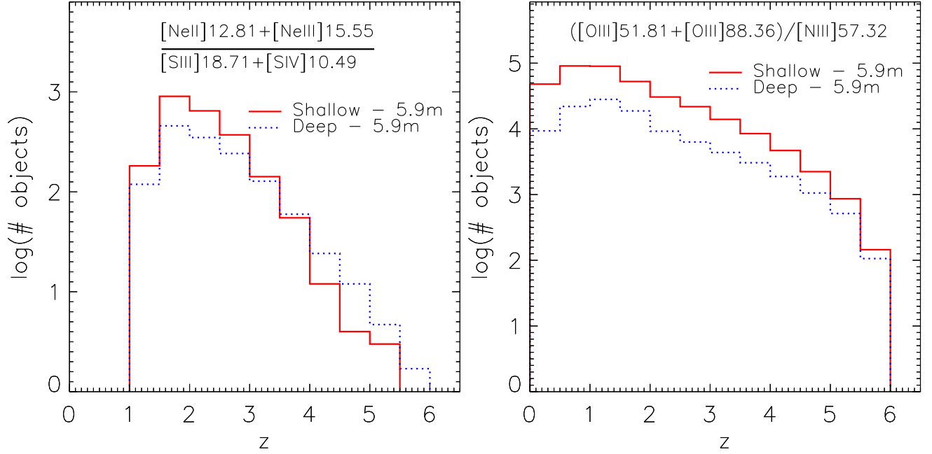
Figure 16. Left panel: predicted redshift distributions of galaxies detected simultaneously in the [NeII] 12.81, [NeIII] 15.55, [SIII] 18.71, and [SIV] 10.49 \mu\text{m} lines by the shallow (10 \text{deg}^2 ) and deep (1 \text{deg}^2 ) surveys with a 5.9 m telescope. Both surveys have a total amount of observing time equal to 1000 h. Right panel: the same, but for the simultaneous detection of the [OIII] 51.81, [OIII] 88.36, and [NIII] 57.32 \mu\text{m} lines.
