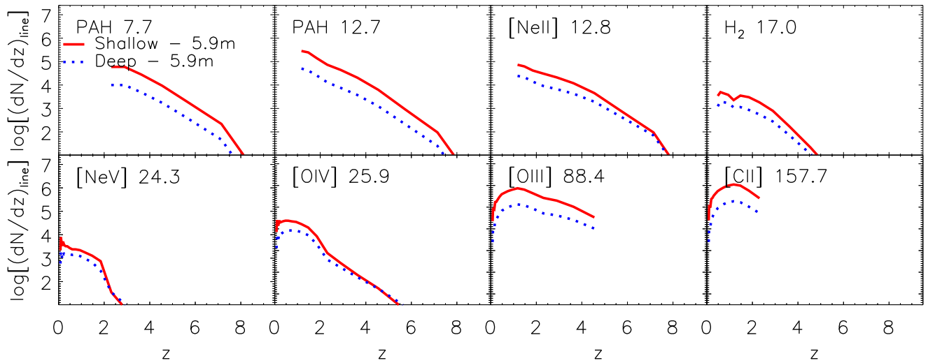
Figure 12. Predicted redshift distributions of galaxies detected in the three brightest AGN lines ([NeV]14.32, [NeV]24.31, and [OIV]-25.89 \mu\text{m} ) and in selected lines indicating star formation, namely those with relatively high detection rates. The predicted distributions pertain to shallow (solid red lines, 10 \text{ deg}^2 areal coverage) and deep (dotted blue lines, 1 \text{ deg}^2 areal coverage) surveys, each conducted in 1000 h of observing time with a 5.9 m telescope.
