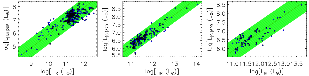
Figure 3. Luminosity of the [NII] 205.2 \mu\text{m} (left panel), [CI] 370.4 \mu\text{m} (central panel) and [CI] 609.1 \mu\text{m} (right panel) lines, versus continuum IR luminosity. The green bands show the 2\sigma range around the mean linear relation \log(L_{\ell}/L_{\odot}) = \log(L_{\text{IR}}/L_{\odot}) + c ; the values of c \equiv \langle \log(L_{\ell}/L_{\text{IR}}) \rangle are given in Table 1. See text for the sources of data points.
