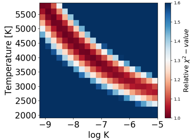
Figure 4. Shown is the abundance-temperature degeneracy for K I line. log K denotes the logarithmic volume mixing ratio of K. Reduced \chi^2 values (colour marked) relative to the best value compare the observational K I line with various synthetic line profiles. Each pixel corresponds to one comparison.
