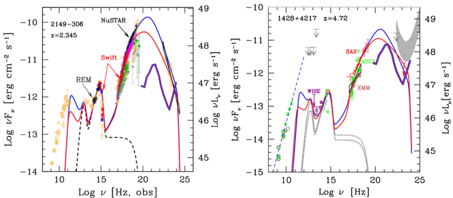
Fig. 6 SED of PKS 2149-306 at z = 2.345 (left panel) and the fitting model by [125] and GB 1428+4217 at z = 4.72 (right panel) and the fitting model by Ghisellini (private communication). Downward arrow is 2\sigma Fermi upper limit over 7.5 years (see [102]). The sensitivity of e-ASTROGAM, calculated for an effective exposure of 1 year, is shown as a purple curve in the 0.3 MeV–3 GeV range. The bulk of the power is expected in the MeV band, around 10^{21} Hz
