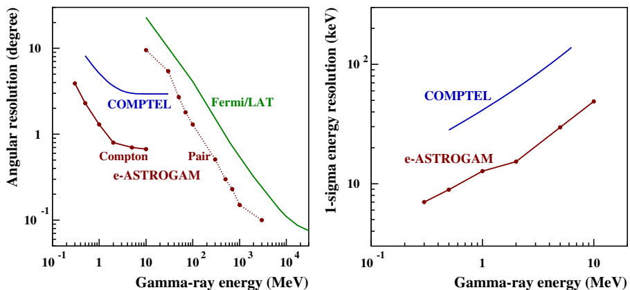
Fig. 19 Left panel —e-ASTROGAM on-axis angular resolution compared to that of COMPTEL and Fermi /LAT. In the Compton domain, the presented performance of e-ASTROGAM and COMPTEL is the FWHM of the angular resolution measure (ARM). In the pair domain, the point spread function (PSF) is the 68% containment radius for a 30^\circ point source. The Fermi /LAT PSF is from the Pass 8 analysis (release 2 version 6) and corresponds to the FRONT and PSF event type. Right panel — 1\sigma energy resolution of COMPTEL and e-ASTROGAM in the Compton domain after event reconstruction and selection on the ARM
