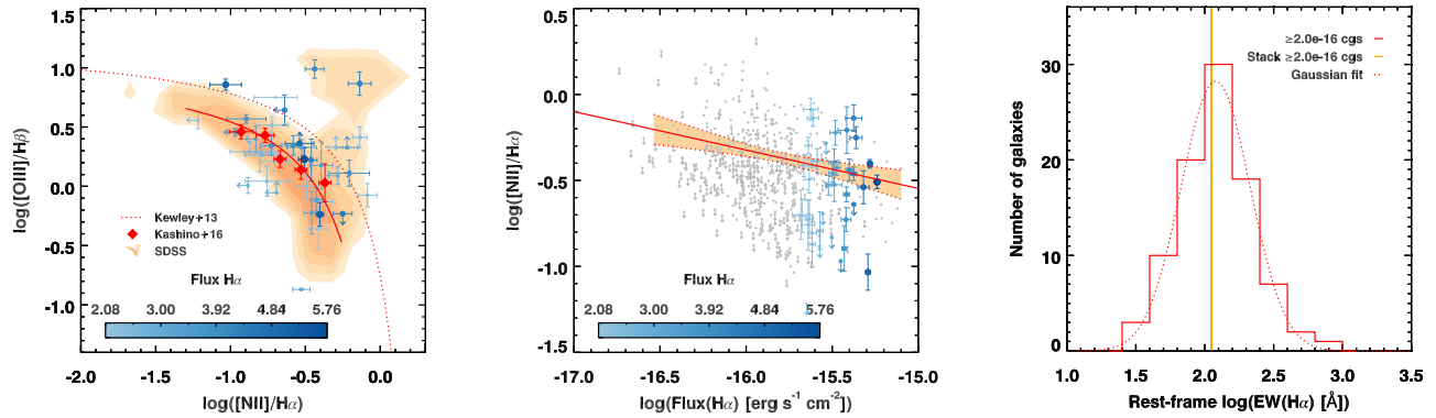
Figure 9. Spectroscopic properties of bright H\alpha emitters at z \sim 1.5 . Left: BPT diagram for spectroscopically confirmed emitters with H\alpha flux \geq 2 \times 10^{-16} \text{ erg cm}^{-2} \text{ s}^{-1} from the FMOS-COSMOS survey. The blue solid circles mark bright emitters. The colour intensity scales as the H\alpha flux in units of 10^{-16} \text{ erg cm}^{-2} \text{ s}^{-1} reported in the colour bar. The red diamonds and solid line mark the average location of the FMOS-COSMOS sample of SFGs with total H\alpha flux \geq 4 \times 10^{-17} \text{ erg cm}^{-2} \text{ s}^{-1} and the best fit by Kashino et al. (2017a). The red dotted line indicates the limiting curve dividing SFGs and AGN at z = 1.55 as parametrized in Kewley et al. (2013). The orange shaded area marks the location of SDSS galaxies with an intrinsic H\alpha luminosity corresponding to a total H\alpha flux of \geq 4 \times 10^{-17} \text{ erg cm}^{-2} \text{ s}^{-1} at z = 1.55 . Centre: [NII]/H\alpha ratios as a function of the total observed H\alpha flux for the spectroscopic FMOS-COSMOS sample. The blue solid circles mark bright H\alpha emitters in the BPT in the left-hand panel. The colour intensity scales as the H\alpha flux in units of 10^{-16} \text{ erg cm}^{-2} \text{ s}^{-1} reported in the colour bar. Grey dots and arrows mark the position of the rest of the FMOS-COSMOS spectroscopic sample described in Kashino et al. (2017a). The red solid line indicates the best fit to the data. The orange area and the red dotted lines mark the 95 per cent confidence limits of the fit. Right: The red histogram shows the distribution of rest-frame \log[EW(H\alpha)] for spectroscopically confirmed emitters with H\alpha flux \geq 2 \times 10^{-16} \text{ erg cm}^{-2} \text{ s}^{-1} . The red dotted line marks the best Gaussian fit to the distribution. The orange band indicates the 1\sigma confidence limit around the value estimated from the stacked spectrum in Fig. 8.
