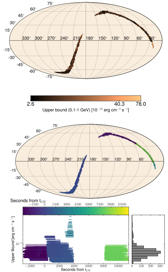
Figure 9. Adaptive time interval analysis for GW151226 over the first Fermi orbit containing t_{\text{GW}} : flux upper bound map during T_{\text{adaptive}} (top), the entry time into the LAT FOV relative to t_{\text{GW}} of the RoI for each pixel within the LIGO localization contour (middle), and the upper bound light curves for each RoI (bottom). The horizontal bars in the bottom panel correspond to the values of the LAT upper bounds, and their position along the time-axis coincides with the interval of time used in the analysis. The color of each bar indicates the time when the RoI entered the LAT FOV, and matches the color of the pixel in the middle panel. The horizontal histogram displays the density of upper bounds.
