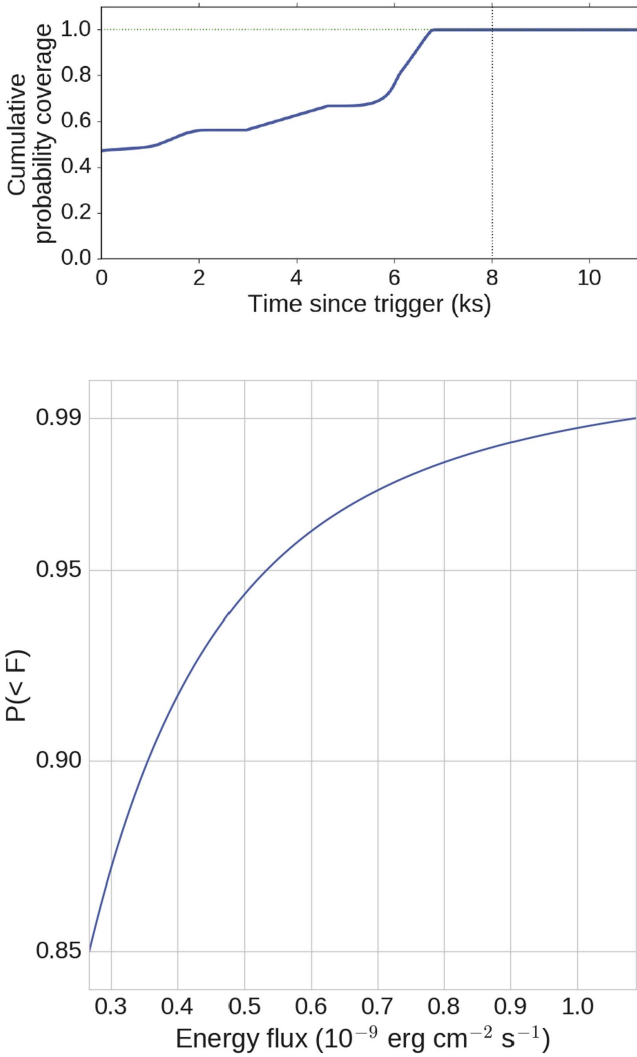
Figure 6. LAT observations of LVT151012: cumulative fraction of the LIGO localization probability observed by the LAT as a function of time since t_{\text{LVT}} (top); integral of the marginalized posterior for the 0.1–1 GeV energy flux (bottom) during the T_{\text{fixed}_2} interval. The flux at which the blue curve intersects a given probability P(F < x) corresponds to the upper bound at that credibility level.
