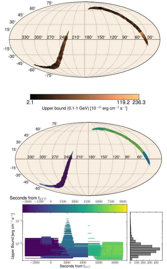
Figure 7. Adaptive time interval analysis for LVT151012 over the first Fermi orbit containing t_{\text{LVT}} : flux upper bound map during T_{\text{adaptive}} (top), the entry time into the LAT FOV relative to t_{\text{LVT}} of the RoI for each pixel within the LIGO localization contour (middle), and the upper bound light curves for each RoI (bottom). The horizontal bars in the bottom panel correspond to the values of the LAT upper bounds, and their position along the time-axis coincides with the interval of time used in the analysis. The color of each bar indicates the time when the RoI entered the LAT FOV, and matches the color of the pixel in the middle panel. The horizontal histogram displays the distribution of upper bounds.
