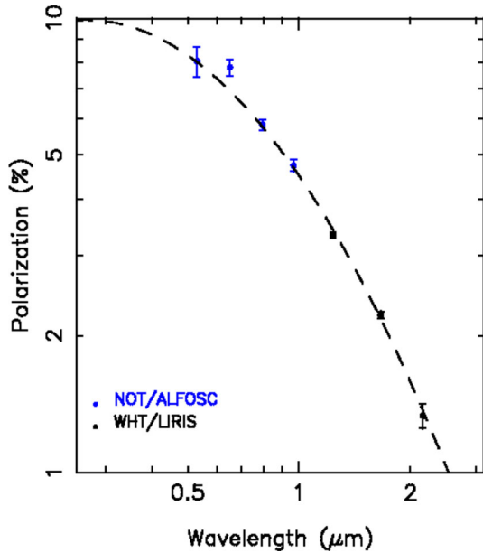
Figure 2. The polarization spectral energy distribution taken during (and near) quiescence. The optical NOT (blue filled circles) were taken on 2016 May 24 (~MJD 57192.20) and near-IR points (black filled circles) were taken on 2015 July 27 (~MJD 57230.43; Section 2.4). The dashed line shows an interstellar polarization model fit to the data.
