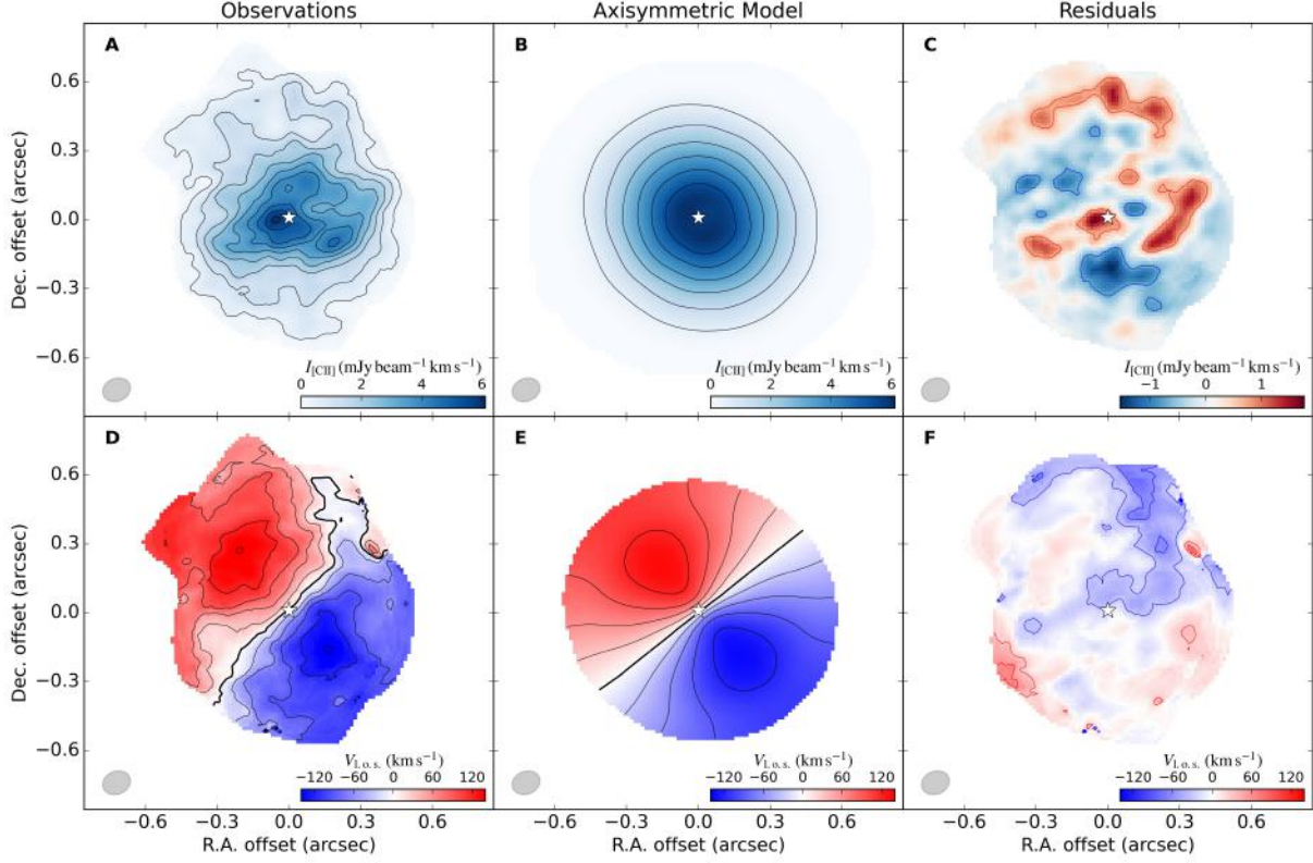
Figure S1: Moment Maps: integrated [C II] intensity ( I_{[\text{CII}]} ) map from the observed ( A ), model ( B ), and residual data cube ( C ); [C II] line-of-sight velocity ( V_{\text{l.o.s.}} ) map from the observed ( D ), model ( E ), and residual data cube ( F ). North is up and east is left. The kinematic centre (R.A. = 03^{\text{h}} 32^{\text{m}} 29.295^{\text{s}} ; Dec. = -27^{\circ} 56' 19.60'' ) is shown with a white star. The beam size is plotted as the grey ellipse in the bottom-left corner. In panels A and B, iso-emission contours range from 0.35 \text{ mJy km s}^{-1} ( \sim 3\sigma ) to 6 \text{ mJy km s}^{-1} in steps of 0.7 \text{ mJy km s}^{-1} . In panel C, residual contours are at -6\sigma (blue) and +6\sigma (red); non-axisymmetric, arm-like features are detected. In panels D and E, iso-velocity contours range from -120 to +120 \text{ km s}^{-1} in steps of 30 \text{ km s}^{-1} ; the bold contour highlights the systemic velocity (set to zero). In panel F, the residual contours are at -60 and -30 \text{ km s}^{-1} (blue) as well as +30 and +60 \text{ km s}^{-1} (red). Non-circular motions above the velocity resolution ( \sim 30 \text{ km s}^{-1} ) are detected along an arm-like feature towards the northwest (see also Fig. S4).
