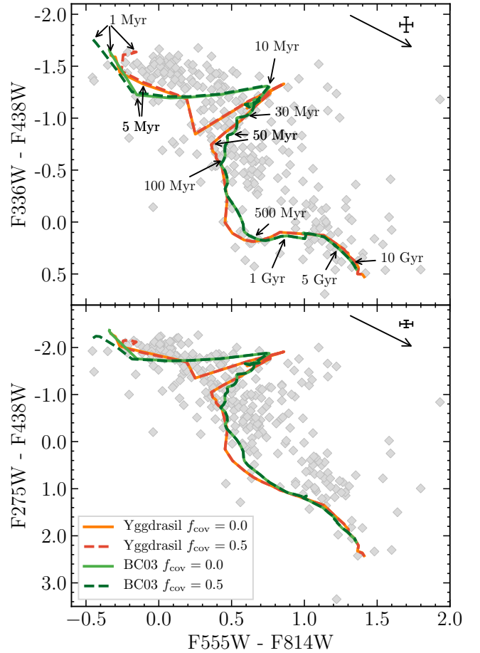
Figure 5. Top: F336W - F438W vs F555W - F814W ( U-B vs V-I ) color-color diagram for a collection of theoretical single-age stellar population models, along with the PHANGS–HST stellar clusters for NGC 3351. Magnitudes are in the Vega system. The stellar clusters have been aperture corrected as well as corrected for foreground Milky Way extinction. The BC03 (green) and YGGDRASIL (orange) tracks are shown both with (dashed) and without (solid) nebular emission. The y-axis has been flipped so the top left-hand corner of the diagram is the ‘bluest’ and the bottom right-hand corner is the ‘reddest’. The top panel annotates various ages along the SSP tracks; ages where the tracks deviate significantly from each other are pointed out with two arrows. The class 1 and 2 star clusters are plotted in grey. Both panels include a reddening vector for A_V = 1 mag as well as a typical error bar for the cluster photometry computed from the median uncertainty in the colors. Bottom: Same as the top panel except with F275W ( NUV ) instead of F336W ( U ).
