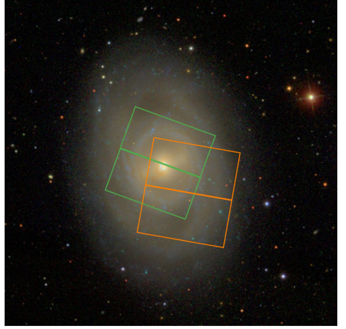
Figure 1. WFC3 observation footprints from PHANGS–HST (green) and LEGUS (orange) overlaid on a Sloan Digital Sky survey g-r-i image of NGC 3351 (David W. Hogg, Michael R. Blanton, and the Sloan Digital Sky Survey Collaboration). The WFC3 field of view is 162'' \times 162'' .
