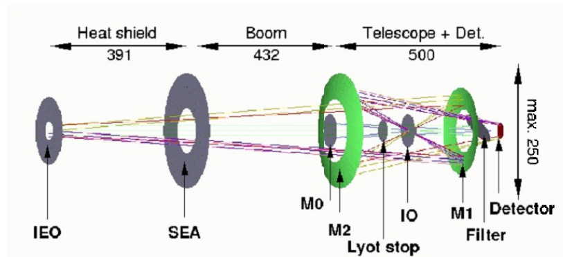
Figure 1 Optical layout of METIS.
