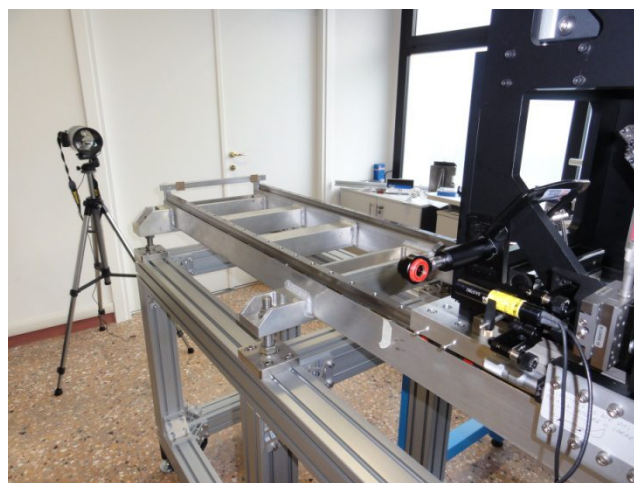
Figure 7 Optical setup utilized for the measurement of the angular deviation of the ISVL carriage along its stroke.
