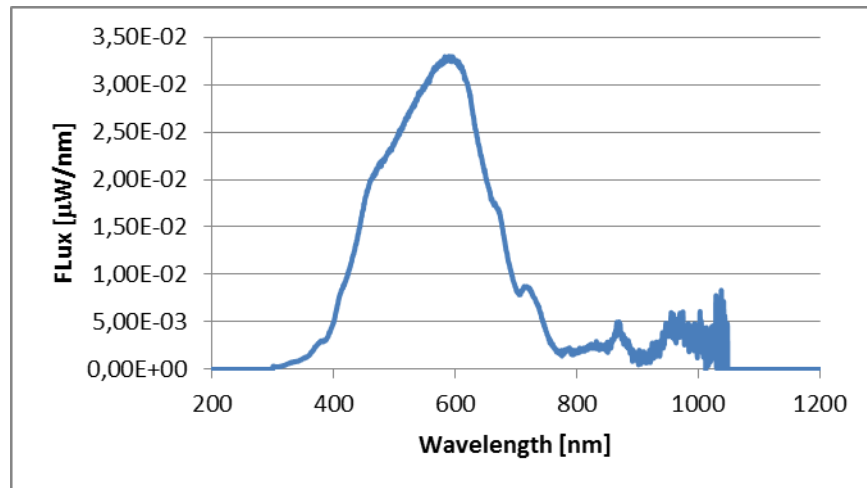
Figure 13 Flux spectral distribution measured with the calibrated system.
