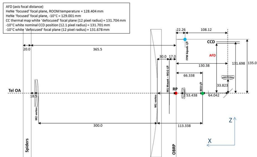
Figure 2. Scheme of the model at Room Temperature.
