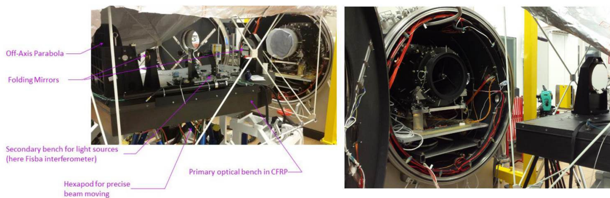
Figure 8. TEL in horizontal position in front of the OGSE (Left). TEL into the thermal vacuum chamber (Right).
