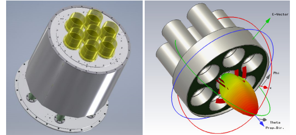
Fig. 6. Left: Arrangement of the array inside the cryostat showing the seven feeds. Right: 3D view of the S-band seven-beam receiver with absorbers surrounding the feeds (in dark colour), showing the radiation pattern from the central feed.
