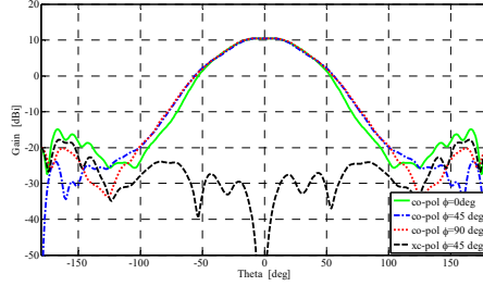
Fig. 9. Radiation pattern of array central feed with absorber at 4.50 GHz.
