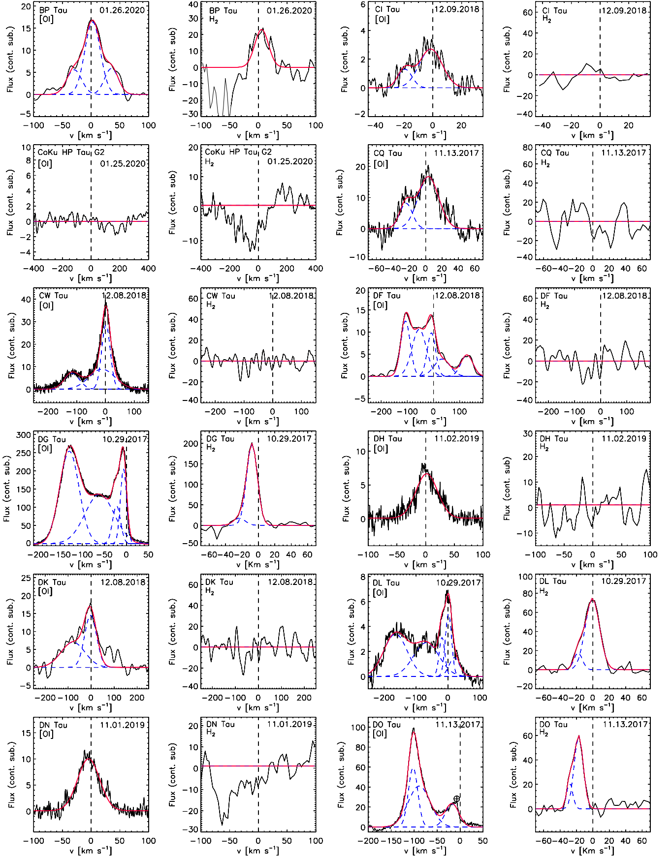
Fig. A.1. Continuum-subtracted [O I] and H 2 line profiles. In red we plot the fit to the profile, obtained by adding single or multiple Gaussians (dashed blue lines). Flux units are 10^{-15} \text{ ergs}^{-1} \text{ cm}^{-2} \text{ \AA}^{-1} . For each panel, we indicate the target name and date of observation (MM.DD.YYYY).
