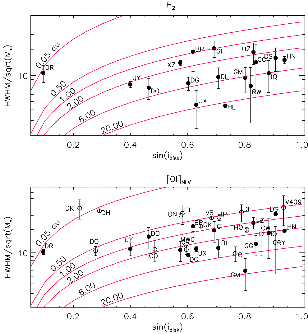
Fig. 8. Half-width at half maximum divided by the square root of the stellar mass for the H_2 (top) and [O I]_{NLV} (bottom) NLVC as a function of the sine of the disk inclination. Keplerian models for gas emitted from disk radii of 0.05, 0.50, 1.00, 2.00, 6.00, and 20.00 au are shown as solid red lines. Bottom panel: empty circles refer to stars whose H_2 profile is not detected.
