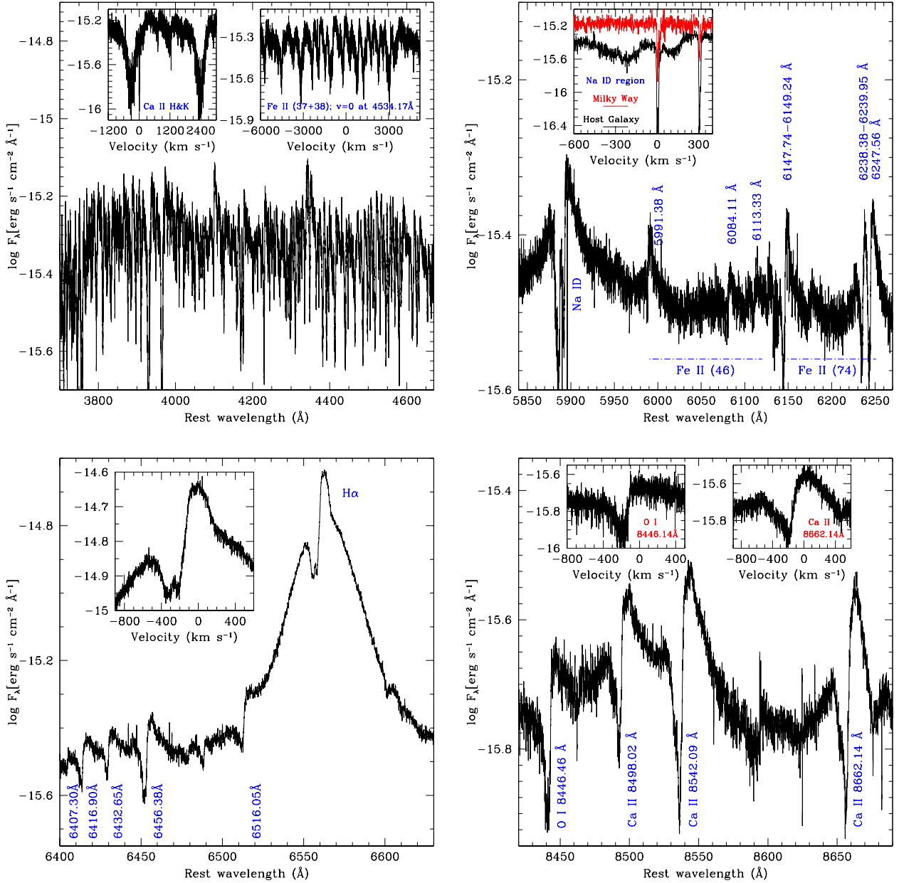
Fig. 4. High resolution UVES spectrum at -5 d. Top left: blue region (3700–4670 Å) dominated by Fe II lines. The insets show blow-ups of the Ca II H&K region (centred at \lambda 3933.66 ) and the Fe II (multiplets 37 and 38; centred on the \lambda 4534.17 line). Top right: region between 5840 Å and 6270 Å with Na ID and Fe II lines (multiplets 46 and 74). The inset shows the narrow Na ID interstellar doublet centred on the \lambda 5889.95 line; the upper red line is the Milky Way component; the lower black line one is the host galaxy ones). Bottom left: H \alpha region, including also some Fe II lines. The blow-up shows a detail of the narrow H \alpha P Cygni. Bottom right: 8420–8690 Å region with insets showing a detail of O I \lambda 8446.46 (left) and Ca II \lambda 8662.14 .
