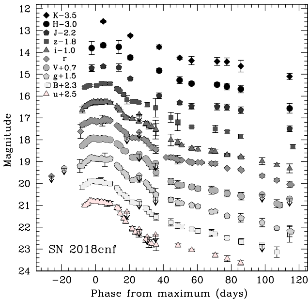
Fig. 5. Optical and NIR light curves of SN 2018cnf.
