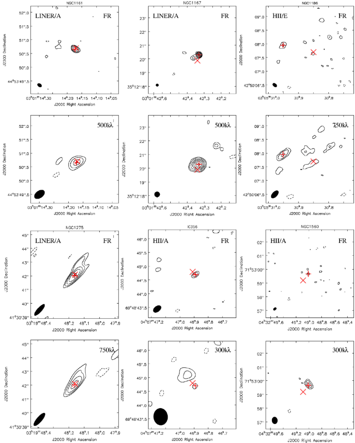
Figure 2. e -MERLIN 1.5-GHz radio maps of the detected and core-identified galaxies. For each galaxy two panels are shown. The upper panel depicts the full-resolution map, while the lower panel shows the low-resolution map obtained with a uv -tapered scale written in the panel (in k\lambda ), all on a same physical scale. For four galaxies (NGC 3516, NGC 4036, NGC 5322, and NGC 5548) a third radio map is presented corresponding to a lower resolution map (see the scale and map parameters in Table 4). The restoring beam is presented as a filled ellipse at one of the corners of each of the maps. The contour levels of the maps are presented in Table 4. The \times marks indicate the optical galaxy centre taken from NED, while the + symbol marks the radio core position, if identified. In the upper panels, the optical (LINER, Seyfert, H II, and ALG) and radio (A, B, C, D, E, see Section 4.2 for description) classifications of the sources are reported. The full sets of figures are available online.
