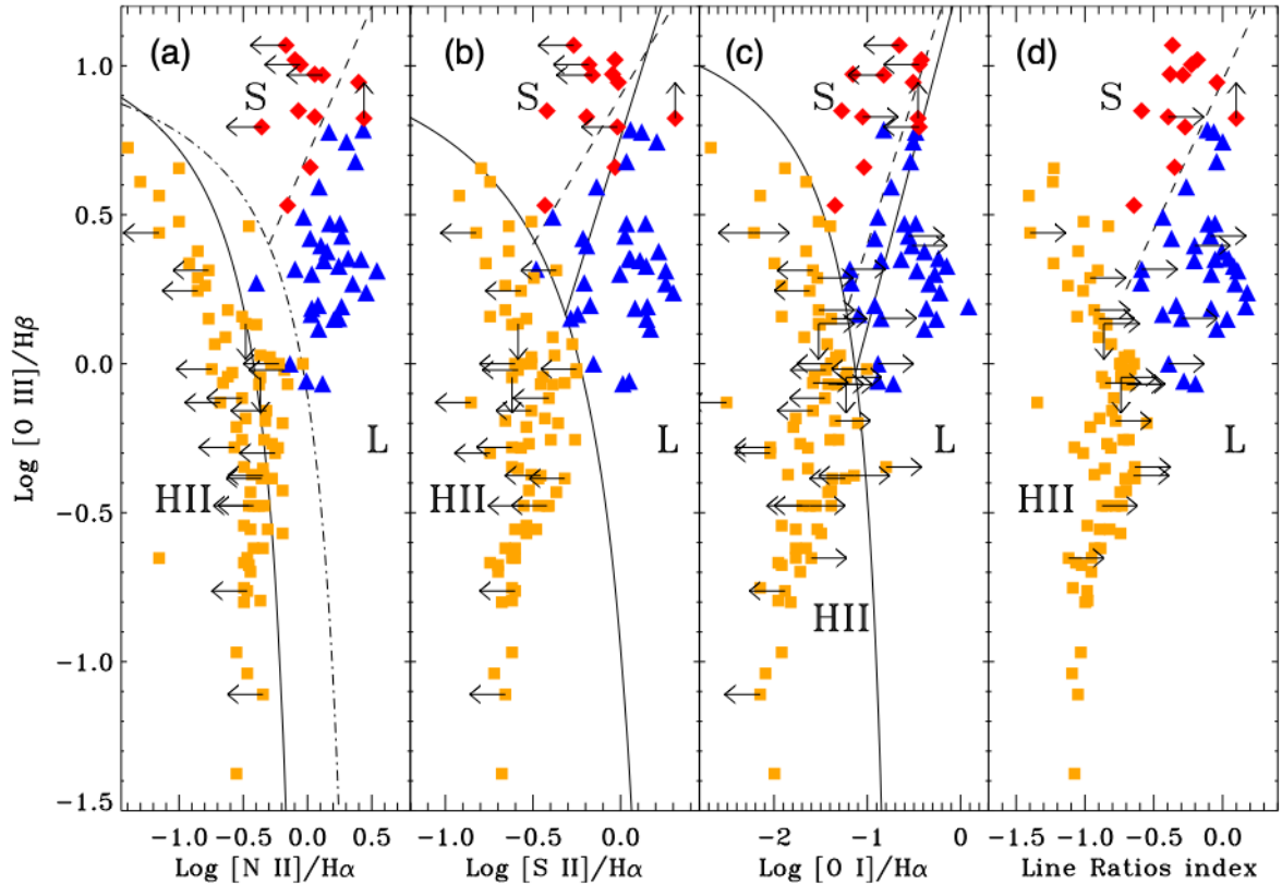
Figure 1. Diagnostic diagrams based on optical spectra (named BPT, Baldwin, Phillips & Terlevich 1981): \log([O III]/H\beta) versus (a) \log([N II]/H\alpha) , (b) \log([S II]/H\alpha) , (c) versus \log([O I]/H\alpha) , and (d) line ratios index (the averaged line ratios, see the definition in Paper I). The data-points represent the 122 galaxies with emission line data taken from Ho et al. (1997) (the remaining 55 sources were classified based on data from the recent literature; see Table 1). In the first three panels, the solid lines separating H II galaxies, LINER, and Seyferts are taken from Kewley et al. (2006). The dashed lines between Seyferts and LINERs in the four panels separate the two classes according to the scheme introduced by Buttiglione et al. (2010). In panel (a), the sources between the solid and the dot-dashed lines were classified as transition galaxies by Ho et al. (1997), which we re-classify as LINER or H II galaxies based on the other diagrams ('b' and 'c'). We mark LINERs as blue triangles, Seyferts as red diamonds, and H II galaxies as orange squares. Several galaxies have different classifications with respect to those from Ho et al. (1997) because of the updated diagnostic diagrams (see Table 1).
