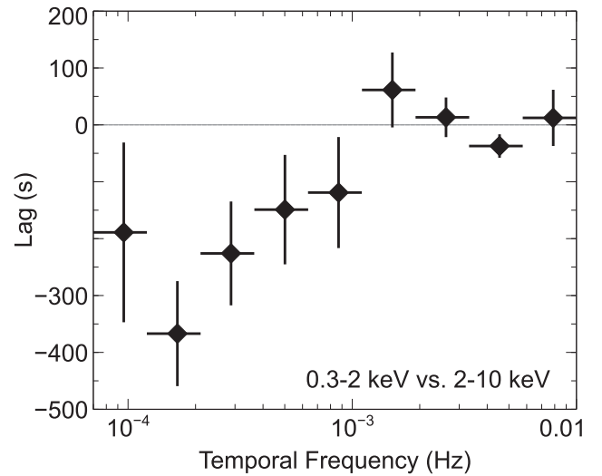
Figure 2. The soft (0.3–2 keV) versus hard (2–10 keV) lags as a function of temporal frequency. By convention, negative lags are soft band lags. The variability on time-scales of thousands of seconds show a soft band lag of ~150 s. This is the third ULX to exhibit soft lags.
