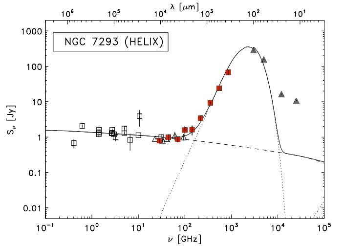
Fig. 9. Model of the SED of NGC 7293 (continuous line) considering both free-free (dashed line) and thermal dust emission (dotted line). Ancillary radio measurements, obtained with different instruments, are shown as open squares (reference numbers given in Table 1: 2, 3, 6, 7, 16, 17, 18, 19, 23, 29 and 52), WMAP 7-year data as open triangles, aperture photometry from IRIS as filled triangles, and Planck data are shown as red squares. IRIS data at 12 \mu\text{m} and 25 \mu\text{m} , which are contaminated by emission lines, are also shown in the plot for completeness, but were not considered in the fitting procedure (see text).
