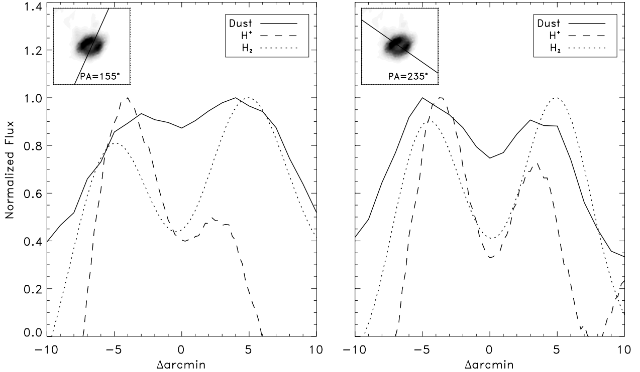
Fig. 14. Profiles of the brightness of the dust ( Planck at 857 GHz – continuous line), radio (H + , NVSS at 1.4 GHz – dashed line) and H 2 (dotted line) components obtained at PA = 155° (left) and 235° (right). Profiles have been normalized to the Helix peak of each maps.
