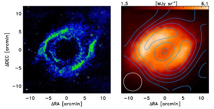
Fig. 13. Left: \text{H}_2 map of the Helix (Hora et al. 2004). Right: the comparison between the \text{H}_2 map (contours) and the Planck 857 GHz map. Only the main-ring emission of the dust component has been reproduced. The \text{H}_2 map has been smoothed to the angular resolution of the Planck map, indicated in the left-bottom corner.
