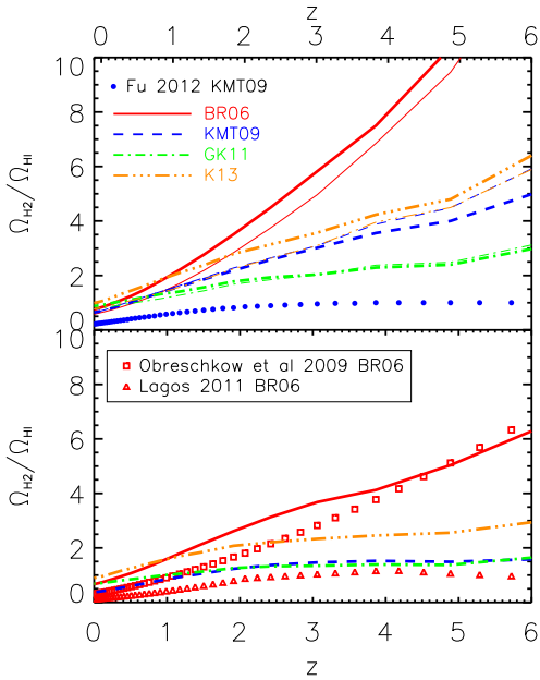
Figure 14. The cosmic molecular ratio \Omega_{H_2}/\Omega_{HI} as a function of redshift. Thick curves correspond to our runs based on the MSII, while thin curves correspond to the MS. The red squares, red triangles, and blue dots are predictions from Obreschkow & Rawlings (2009a, with BR06), Lagos et al. (2011a, with BR06), and Fu et al. (2012, with KMT09), respectively. The top panel shows results for galaxies above M_* > 10^9 M_\odot . The bottom panel shows results for galaxies with M_* > 10^8 M_\odot .
