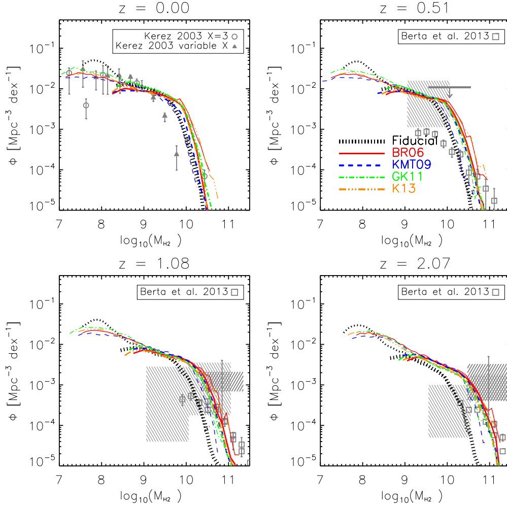
Figure 8. H_2 mass function at redshift z = 0 , z \sim 0.5 , z \sim 1 , z \sim 2 . Thicker lines are used for the MS, while thinner lines correspond to the MSII. The observational measurements at z = 0 are from Keres, Yun & Young (2003). Open circles correspond to the case X_{CO} = 3 , while triangles correspond to a variable X_{CO} . Open squares at higher redshift are from Berta et al. (2013). They are based on indirect estimates of the molecular mass, and include only normal star forming galaxies. Gray shaded regions are based on blind CO detections by Walter et al. (2014), and Decarli et al. (2016) and assume \alpha_{CO} = 3.6 M_{\odot} (K km s^{-1} pc^{-2})^{-1} .
