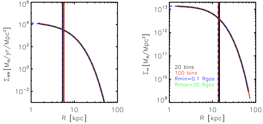
Figure 1. Star formation (left panel) and HI (right panel) surface density profiles for one particular galaxy at z = 0 in different runs. These correspond to a number of bins larger (red) than our default choice (black), smaller inner radius (blue), and larger outer radius (green). This figure refers to the BR06 model, but results are similar for the other models considered. The vertical lines mark the effective radius.
