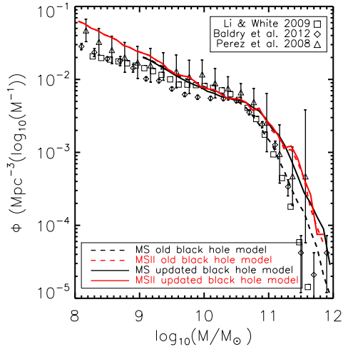
Figure B1. Stellar mass functions based on the MS (black lines) and the MSII (red lines). Dashed lines correspond to the model introduced in Hirschmann, De Lucia & Fontanot (2016, the FIRE feedback scheme), while solid lines correspond to the same physical model including the updates described in Sections 2.2 and 2.3 for the disk size and black hole model.
