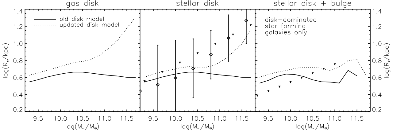
Figure A1. The size-mass relation predicted by the model described in HDLF16 using its original prescriptions for disk sizes (solid lines), and our updated model (dotted lines). The left and middle panels show the half-mass radius for the gaseous and stellar disks, respectively. The right panel shows the half-mass radius of stars, considering both the bulge and disk components, for disk-dominated, star forming galaxies only ( sSFR > 0.3/t_H , M_{bulge}/M_* < 0.5 ). The diamonds with error bars and triangles in the middle panel are observed stellar disk sizes based on SDSS and GAMA (Dutton et al. 2011; Lange et al. 2016, half-light radius for disk only). The triangles are observed sizes based on GAMA data (Lange et al. 2015, half-light radius for disk and bulge).
