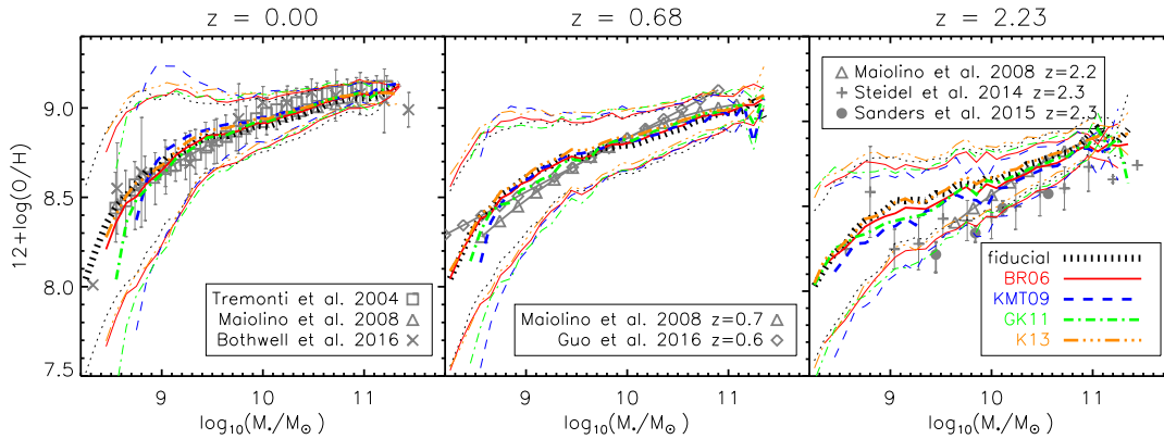
Figure 10. The relation between the cold gas metallicity and galaxy stellar mass. Gray symbols with error bars show observational measurements, while colored lines correspond to the different star formation laws considered in this study. We only select star forming galaxies ( sSFR > 0.3/t_H ), without a significant AGN ( M_{BH} < 10^6 M_\odot ), and with cold gas fraction M_{gas}/(M_{gas} + M_*) > 0.1 . In Tremonti et al. (2004), they used a Kroupa (2001) IMF to calculate stellar mass. We shift it to a Chabrier IMF by dividing the observed masses by a factor 1.06. Thin lines in each panel show the scatter predicted for the BR06 model (the scatter has similar amplitude for the other star formation laws).
