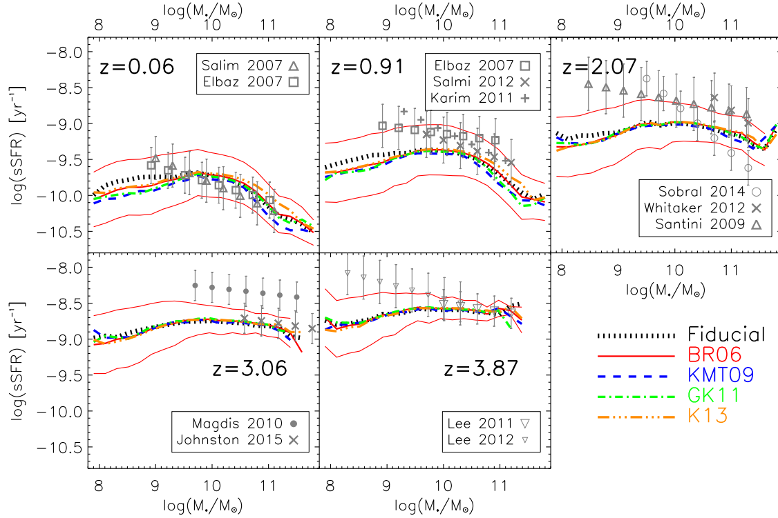
Figure 11. Specific star formation rate as a function of galaxy stellar mass at different redshifts, as labeled. Gray symbols show different observational estimates (Elbaz et al. 2007; Salim et al. 2007; Salmi et al. 2012; Santini et al. 2009; Sobral et al. 2014; Magdis et al. 2010; Johnston et al. 2015; Lee et al. 2011, 2012). All SFR and stellar mass estimates are converted to a Chabrier IMF, to be consistent with our model assumptions. Thick lines show the mean relation obtained for all star formation laws considered in our work, while the thinner lines in all panels show the scatter (standard deviation) predicted for the BR06 model (the other models exhibit a similar scatter).
