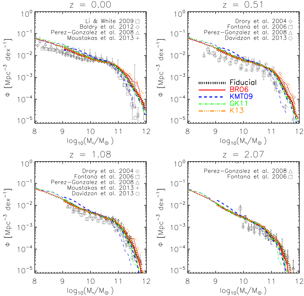
Figure 6. Galaxy stellar mass functions at redshift z = 0 , z \sim 0.5 , z \sim 1 , and z \sim 2 . Gray symbols show different observational estimates (Li & White 2009; Baldry et al. 2012; Pérez-González et al. 2008; Moustakas et al. 2013; Drory et al. 2004; Fontana et al. 2006; Davidzon et al. 2013), while lines of different colours and types correspond to different star formation laws, as indicated in the legend. Thicker lines are used for the MS, while thinner lines correspond to the MSII.
