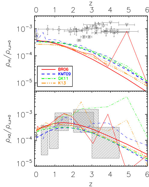
Figure 13. The cosmic density evolution of HI (top panel) and H 2 (bottom panel). Different colours and line styles correspond to the different star formation laws considered in our study, as indicated in the legend. Thick lines correspond to densities estimated considering all galaxies down to the completeness limit of the MSII. Thin lines have been obtained by fitting the HI and H 2 mass functions at different redshifts and extrapolating them towards lower masses (see text for details). Gray symbols and shaded regions show observational estimates.
