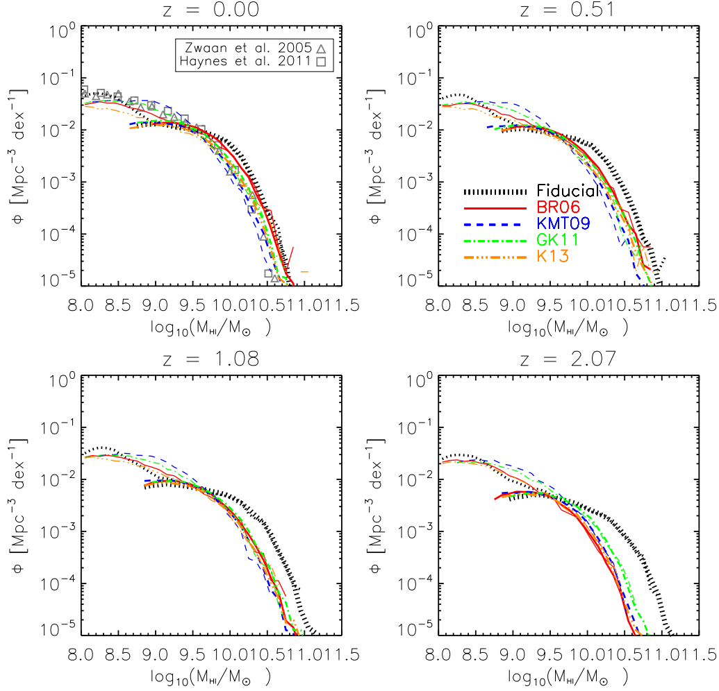
Figure 7. HI mass function at redshift z = 0 , z \sim 0.5 , z \sim 1 , z \sim 2 . Gray triangles and squares show the observational measurements by Zwaan et al. (2005) and Haynes et al. (2011), respectively. Thicker lines are used for the MS, while thinner lines correspond to the MSII.
