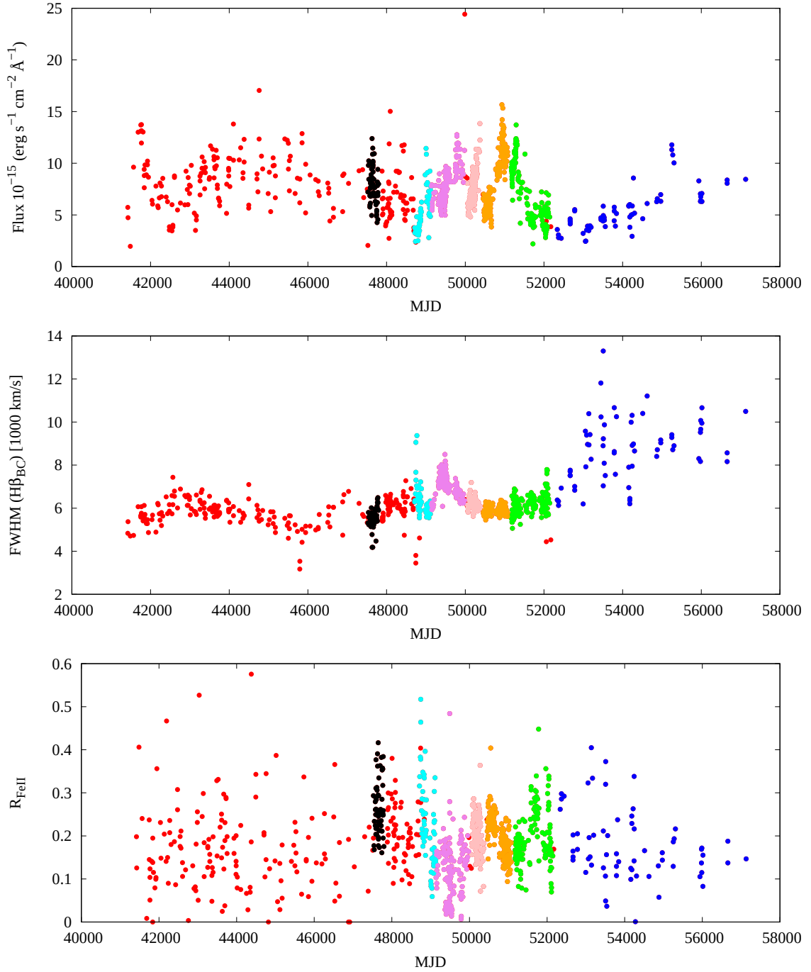
Figure 1. Variability in the NGC 5548 spectra: (top) The light curve of the continuum measured at 5100 Å; (middle) FWHM Hβ variations; (bottom) R_{\text{FeII}} change with the time. Colors correspond to different time intervals.
