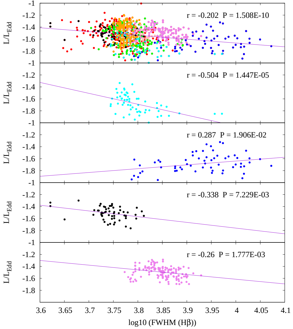
Figure 5. L/L_{Edd} vs \log_{10}(FWHM) trends for long term (top panel) and short term variations (mid and bottom panels). Correlation coefficients are marked on each plot. Colors correspond to those presented in Fig. 1 and Fig. 2.
