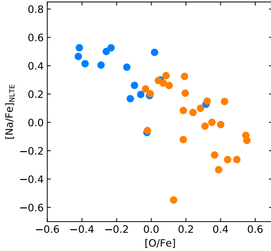
Fig. 11. [Na/Fe] in respect to [O/Fe]. The meanings of symbols are the same as in Fig. 8.
