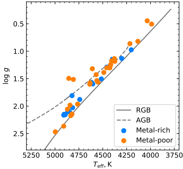
Fig. 4. \log g , T_{\text{eff}} diagram of the investigated NGC 1851 stars together with the PARSEC (Bressan et al. 2012) isochrone of the mean Age = 12.27 Gyr (Valcin et al. 2020) and [Fe/H] = -1.0.
