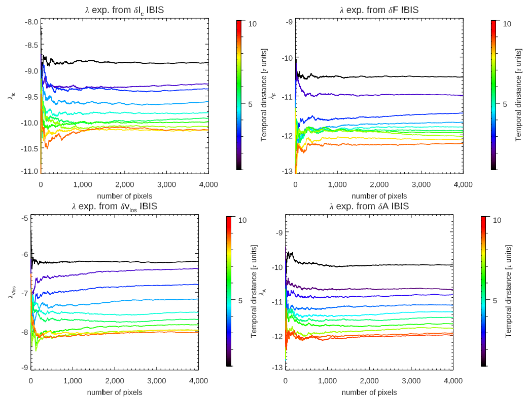
Figure 9. \lambda exponents estimated from the residuals of I_c (top left), v_{LoS} (bottom left), FWHM (top right), and A (bottom right) between maps derived from observations taken at different times. The various colors show results achieved by comparing observations taken at increasing regular time intervals in the time series of IBIS data, expressed in multiples of the temporal cadence \tau (48 s).
