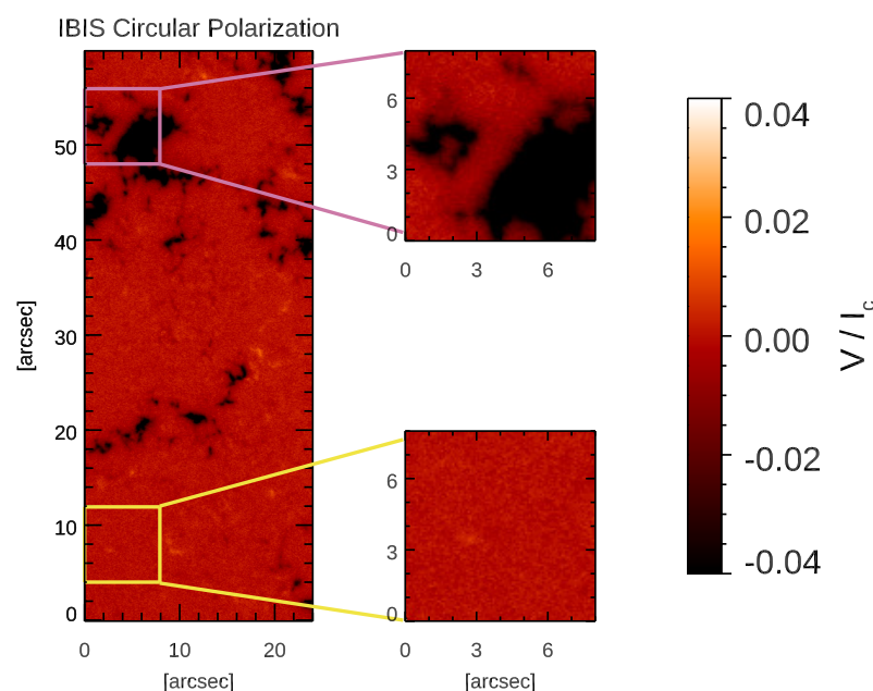
Figure 3. Circular polarization (CP) map relevant to the IBIS data set and the magnifications of the magnetic and quiet selected regions.
