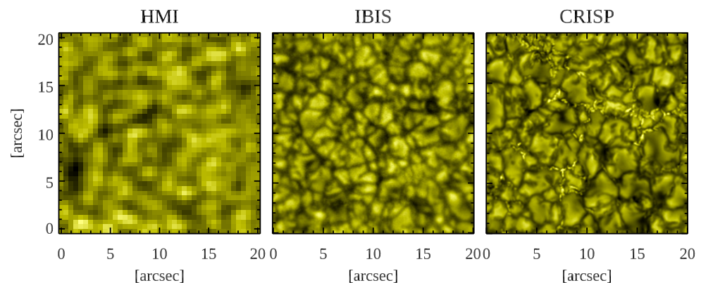
Figure 2. Zoomed regions relevant to the 20'' \times 20'' areas indicated at the center of each panel of Figure 1.
