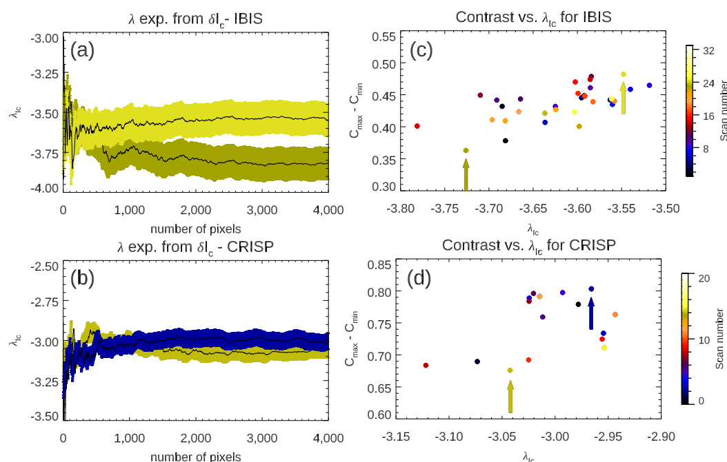
Figure 5. Left: \lambda exponents from \delta I_c fluctuations evaluated in the highest and lowest C continuum images of the IBIS (panel a) and CRISP (panel b) series. Right: relationship between image contrast C = C_{max} - C_{min} and \lambda exponents from \delta I_c fluctuations in the IBIS (panel c) and CRISP (panel d) series.
