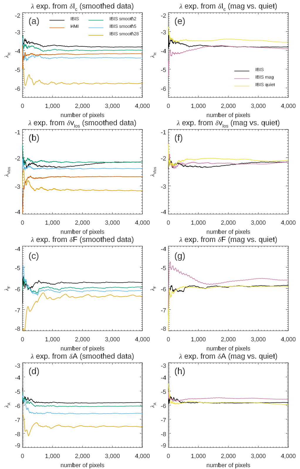
Figure 8. Left: \lambda exponents computed from \delta I_c (a), \delta v_{LoS} (b), \delta F (c), and \delta A (d) fluctuations in the IBIS data smoothed to subgranular ( 2 \times 2 pixel smooth), granular ( 5 \times 5 pixel smooth), and mesogranular ( 28 \times 28 pixel smooth) spatial scales. Right: \lambda exponents evaluated from \delta I_c (e), \delta v_{LoS} (f), \delta F (g), and \delta A (h) fluctuations in the IBIS sub-FoVs representative of magnetic and quiet regions. See text for more details.
