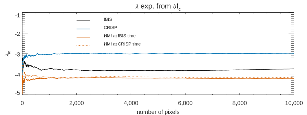
Figure 4. \lambda exponents from \delta I_c fluctuations derived from one continuum intensity image extracted from each of the three analyzed data sets. See text for more details.
