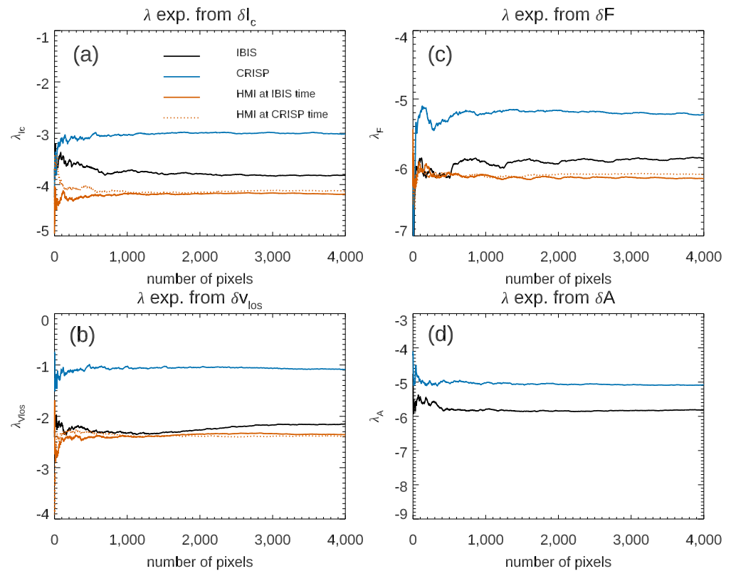
Figure 6. \lambda exponents evaluated from \delta I_c (panel a), \delta v_{LoS} (panel b), \delta F (panel c), and \delta A (panel d) fluctuations for IBIS, CRISP, and HMI data sets.
