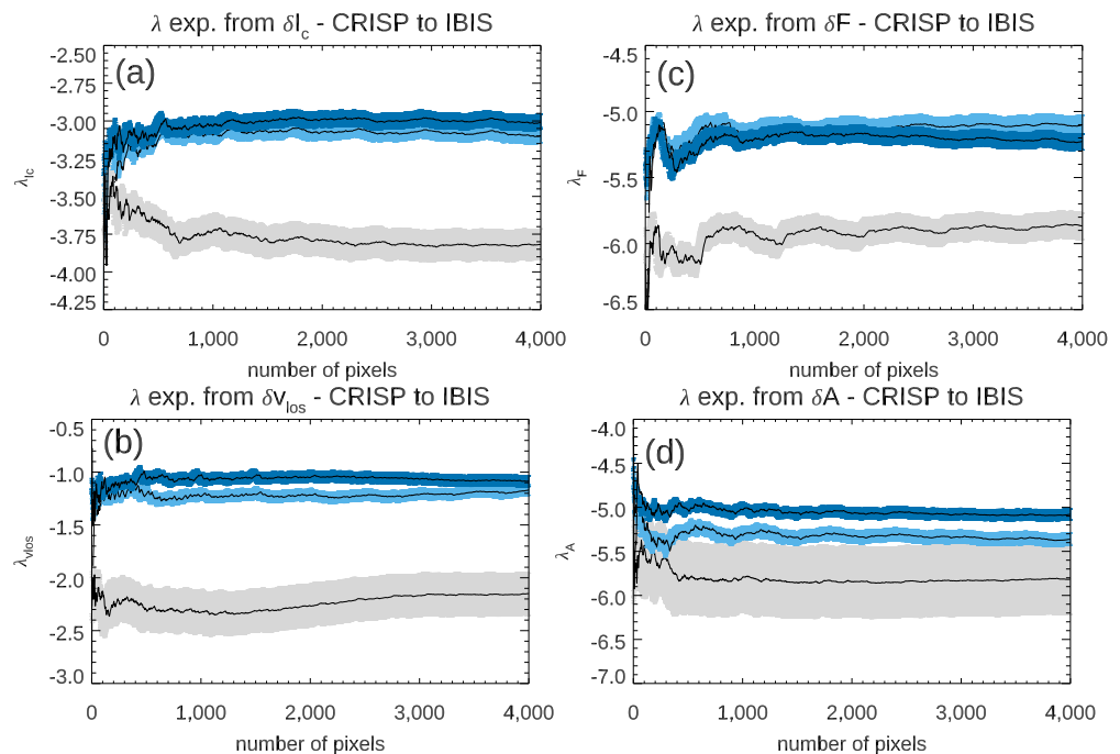
Figure 7. \lambda exponents from \delta I_c (panel a), \delta v_{LoS} (panel b), \delta F (panel c), and \delta A (panel d) fluctuations, by considering the highest contrast scans in the IBIS (gray shaded area) and CRISP (blue shaded area) series, and the CRISP degraded data (light blue shaded area). See text for more details.
