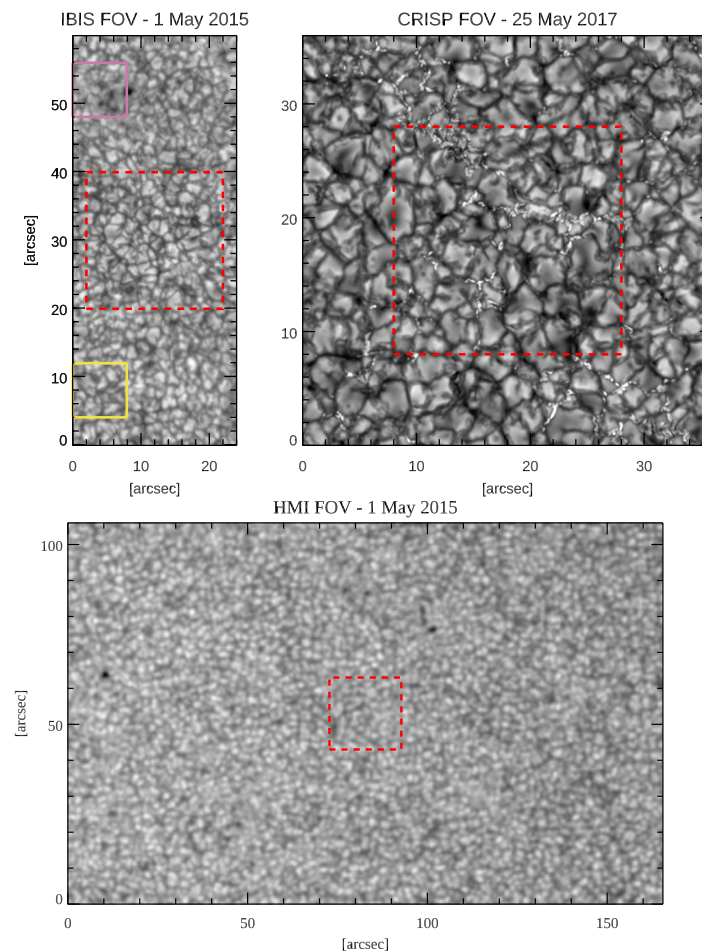
Figure 1. Continuum intensity maps of the three data sets used in this work, for IBIS (top-left panel), CRISP (top-right panel), and HMI (bottom panel) observations. The purple and yellow boxes frame the selected IBIS magnetic and quiet sub-FoVs. The dashed red boxes indicate the 20'' \times 20'' areas as shown in Figure 2. For the sake of conciseness, we only display the HMI data which are co-temporal with IBIS observations. See Section 2 for more details.
