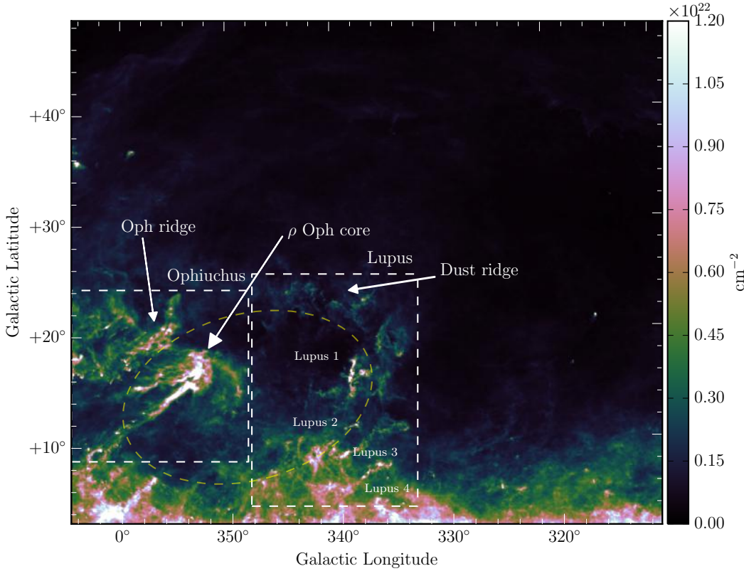
Fig. 1. Total gas column density ( N_H ) map derived from the \tau_{353} Planck map. The white dashed rectangles delimit the Ophiuchus and Lupus dark complexes according to Lombardi et al. (2008a). The yellow dashed ellipse delimits the inner boundary of the bubble.
