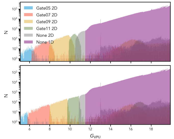
Fig. 2. Distribution of the number of BP/RP observations acquired in BP ( top panel ) and RP ( bottom panel ) with a given gate and WC configuration vs. on-board magnitude labelled as G_{VPU} . The gated observations for sources fainter than \approx 11.5 mag in the G -band are due to occasional alignment of these sources with brighter objects triggering the activation of a gate.
