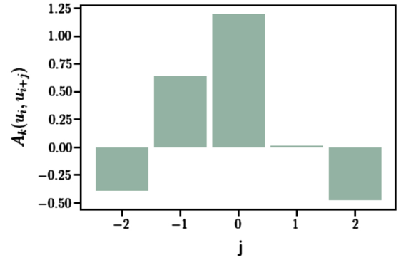
Fig. 6. A_k(u_i, u_{i+j}) values defining the instrument calibration for one specific configuration (RP, CCD row 1, preceding FoV, ungated, 1D) in the time range including OBMT-Rev 5000 evaluated at u_i = 30.0 and AC coordinate 1000.
