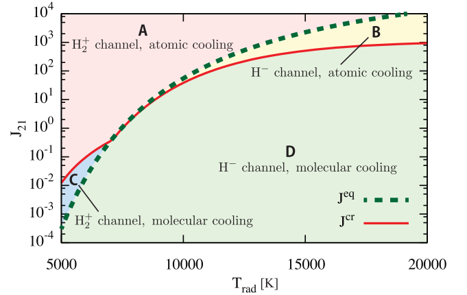
Figure 6. The threshold value J_{21}^{\text{eq}} (dashed green), given by equation (14), above which the H_2^+ channel is more effective than the H^- channel at n_H = 10^2 \text{ cm}^{-3} . The critical intensity J_{21}^{\text{cr}} for the direct collapse shown in Fig. 5 (solid red) is overplotted. The explanation for the domains A–D is given in the text.
