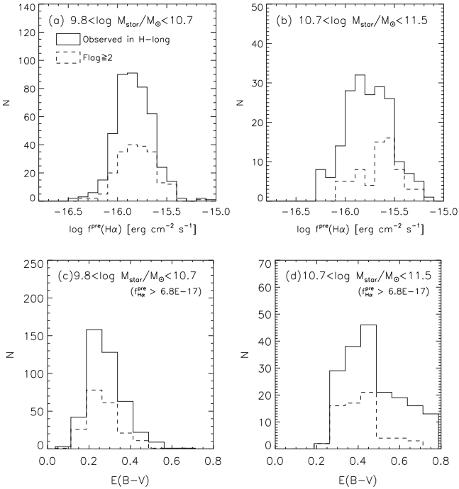
Figure 17. Distribution of spectroscopic redshift successes (quality flag \geq 2 ; dashed histogram) as a function of predicted H\alpha flux (total; i.e., no consideration of the aperture size; panels (a) and (b)) and color excess ( E_{\text{star}}(B - V) ; panels (c) and (d)). The solid black histogram represents the distribution of the full galaxy sample that has been observed with FMOS.
