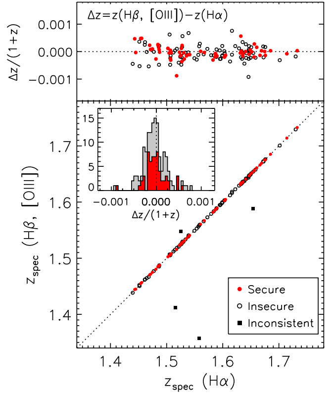
Figure 18. FMOS J -long confirmation of H\alpha -based spectroscopic redshifts. Symbols indicate whether at least one line is detected with a S/N \geq 3 (secure) or not (insecure). Filled squares indicate the insecure redshifts that are in disagreement.
