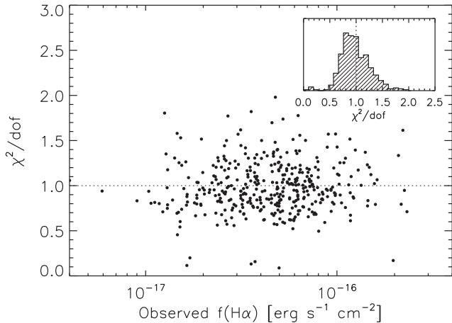
Figure 12. Signal-to-noise estimate of H\alpha using our direct method compared to that based on the errors returned by “MPFITFUN” for an assumed Gaussian line flux profile.
