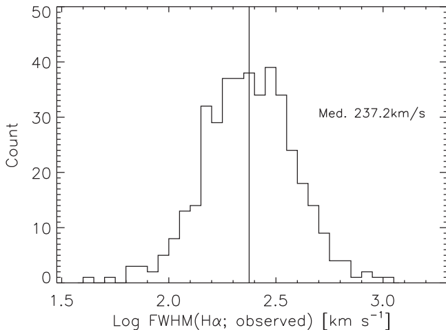
Figure 23. Distribution of the observed \log \text{FWHM} of the \text{H}\alpha line (units of \text{km s}^{-1} ).
