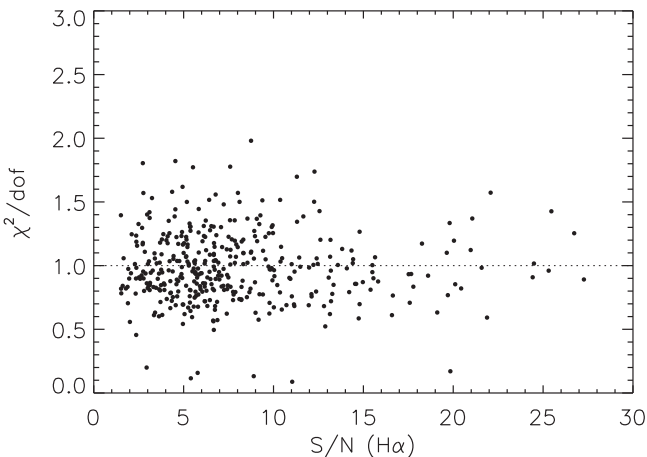
Figure 13. Assessing the accuracy of our line-fitting routine. The reduced chi-square statistic of each fitted H\alpha line as a function of observed H\alpha flux (top panel) and S/N (bottom panel).
