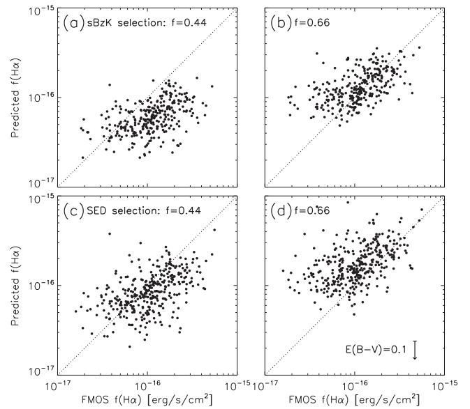
Figure 24. Predicted vs. observed \text{H}\alpha emission-line flux ( f_{\text{H}\alpha} ) with both given as galaxy-wide quantities (i.e., including an aperture correction applied to the observed value). The sample is split into whether the target is included in the sBzK- (a)–(b) or SED-selected (c)–(d) target catalogs. Predicted values are based on the original f -factor of 0.44 (left panels) and our new value f = 0.66 (right panels).
