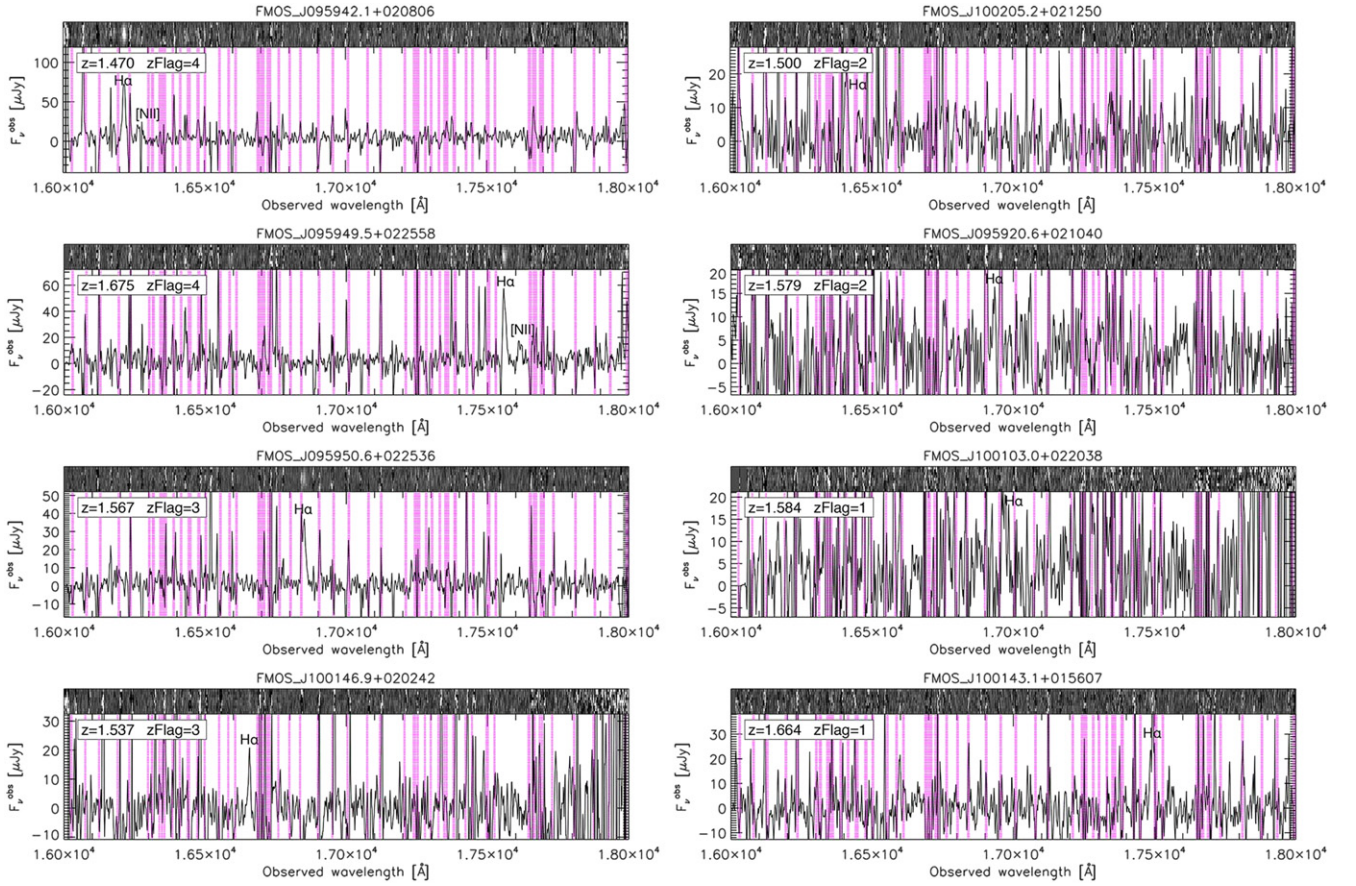
Figure 10. Examples of FMOS H -long spectra (1D and 2D). The H\alpha emission line used to measure the spectroscopic redshift and quality flag is indicated. The vertical bands mask the spectral regions impacted by OH emission.
