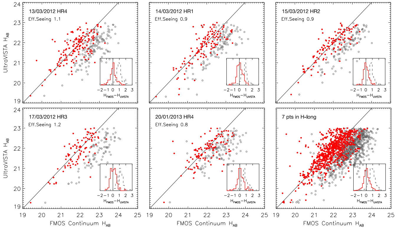
Figure 8. Comparisons of continuum flux observed by FMOS with ground-based photometry (UltraVISTA) for five different H -long observations with varying effective seeing sizes (0.8–1.2). The color of the symbols indicate whether an aperture correction has been applied (red: with correction; gray: no correction). The diagonal lines are linear fits to the corrected photometry. In each panel, a histogram of the difference is shown. The bottom right panel shows the combined sample of seven observations.
