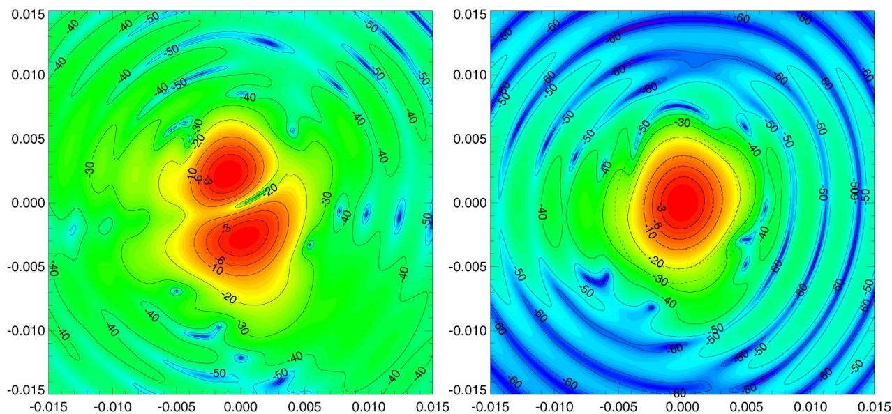
Fig. 4 UV- plot of the x- and co- polar components of LFI19 at 70 GHz, Y- axis polarized.
