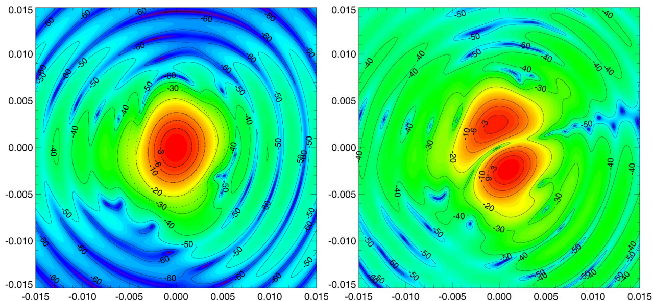
Fig. 3 UV- plot of the co- and x- polar components of LFI19 at 70 GHz, X- axis polarized.
