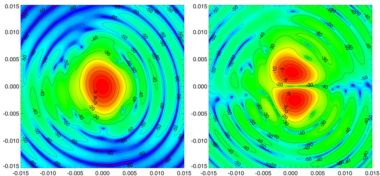
Fig. 7 UV- plot of the co- and x- polar components of LFI21 at 70 GHz, X- axis polarized.
