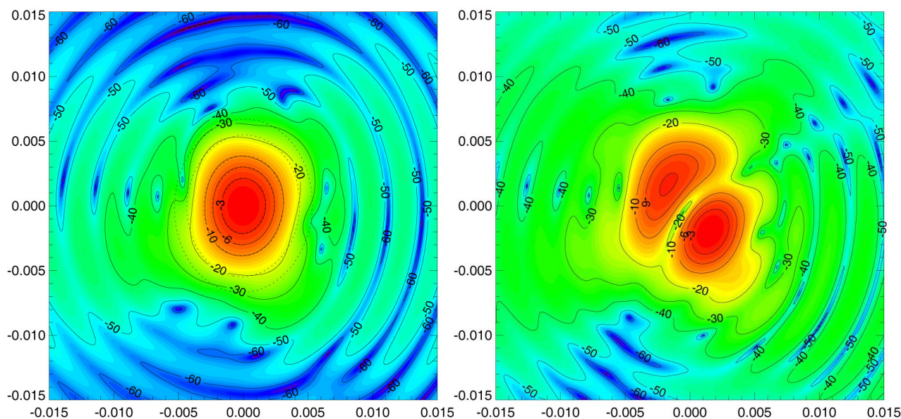
Fig. 1 UV- plot of the co- and x- polar components of LFI18 at 70 GHz, X- axis polarized.
