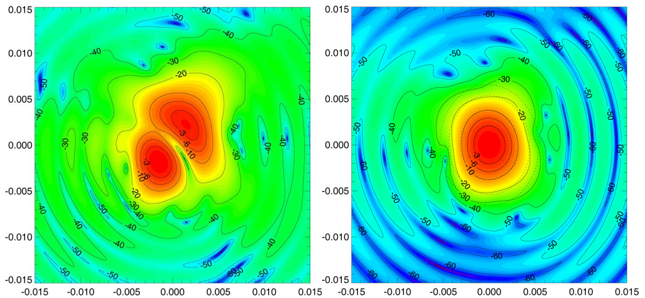
Fig. 12 UV- plot of the x- and co- polar components of LFI23 at 70 GHz, Y- axis polarized.
