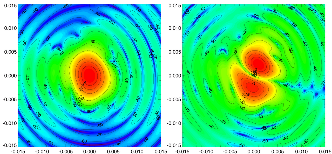
Fig. 9 UV- plot of the co- and x- polar components of LFI22 at 70 GHz, X- axis polarized.
