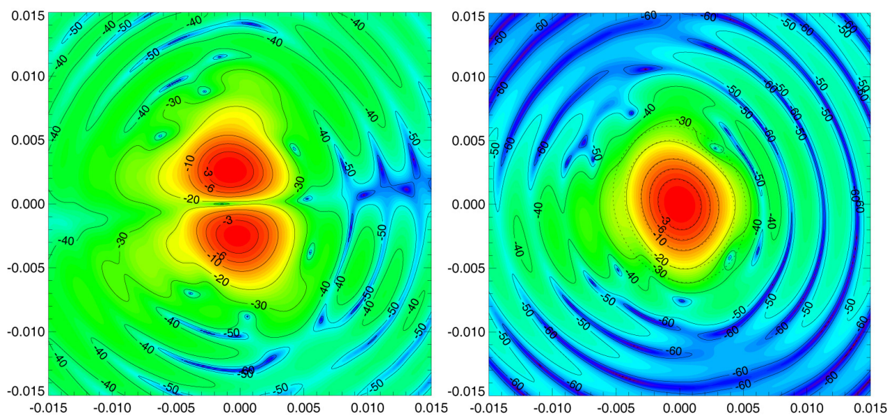
Fig. 8 UV- plot of the x- and co- polar components of LFI21 at 70 GHz, Y- axis polarized.
