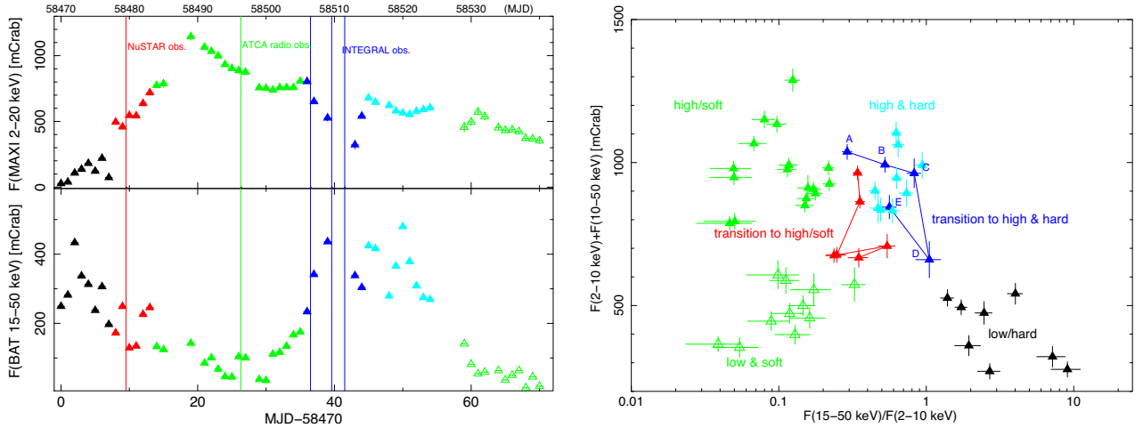
Figure 1. Left-hand panel: the MAXI (upper) and Swift/BAT (lower) light curves of MAXI J1631–479, both with 1-d binning. Vertical lines indicate the time of the NuSTAR , ATCA, and INTEGRAL observations. See text for details. Right-hand panel: the hardness-intensity diagram with each point corresponding to 1 d: on the horizontal axis, we show the ratio F_{(15-50\text{ keV})}^{BAT}/F_{(2-10\text{ keV})}^{MAXI} and in the vertical axis, the total flux F_{(15-50\text{ keV})}^{BAT} + F_{(2-10\text{ keV})}^{MAXI} . Coloured points indicate the different time intervals. Capitals letters indicate the time evolution of the hardness-intensity data during this transition, with A being the starting of the transition and E the end.
