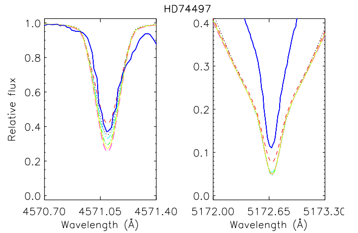
Fig. 8. As in Fig. 5 for HD 74497.
