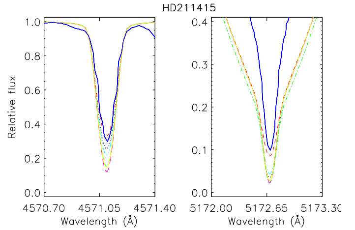
Fig. 7. As in Fig. 5 for HD 211415.
