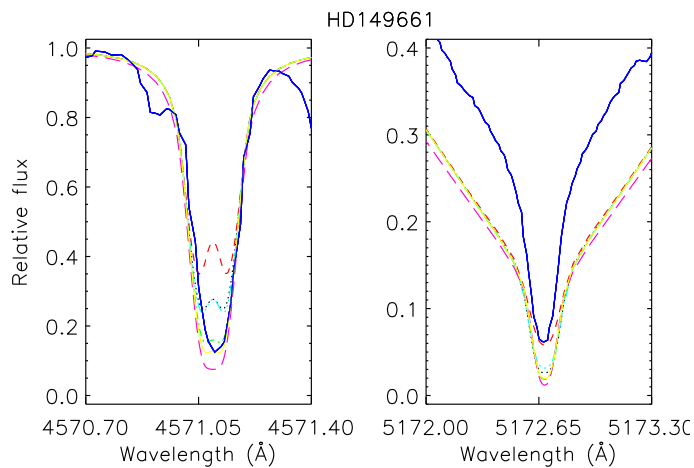
Fig. 10. As in Fig. 5 for HD 149661.
