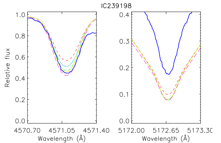
Fig. 9. As in Fig. 5 for IC 2391 98.
