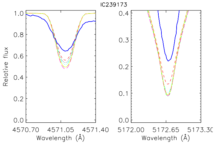
Fig. 6. As in Fig. 5 for IC 2391 73.
