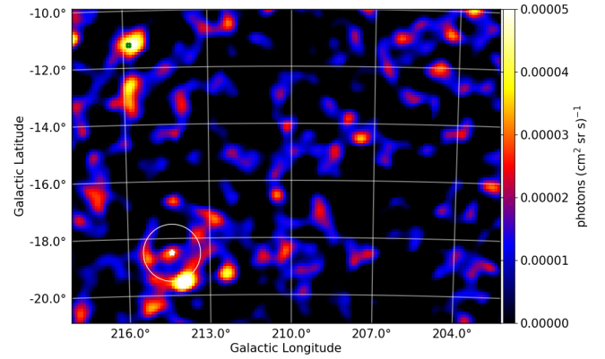
Fig. 3. Residuals of the best fit diffuse emission model to the AGILE map. The white circle shows the ring of \gamma -ray photon excess centred on \kappa Orionis (white star). The green dot on the top-left part of the map highlights the excess of emission corresponding to the unidentified EGRET source 3EG J0616–0720.
