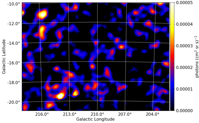
Fig. 5. Residuals of the best fit diffuse emission model to the AGILE map, after including the dark gas tracer C into the calculation.
